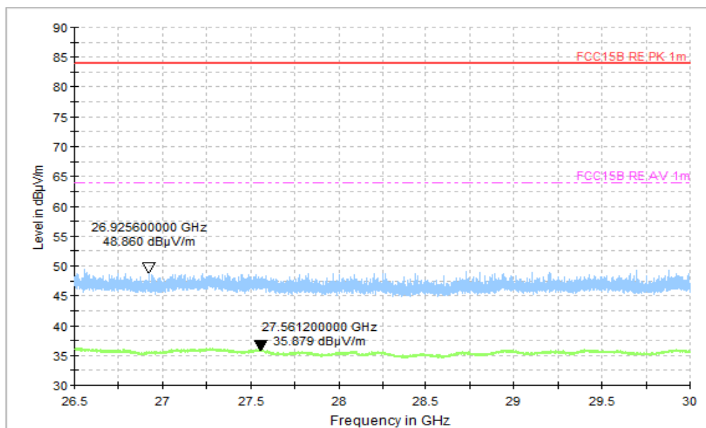
Figure A.1.16. Radiated Emission (Camera,26.5GHz to 30GHz)
