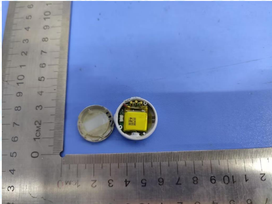
Photo 8 Internal of EUT (L)
