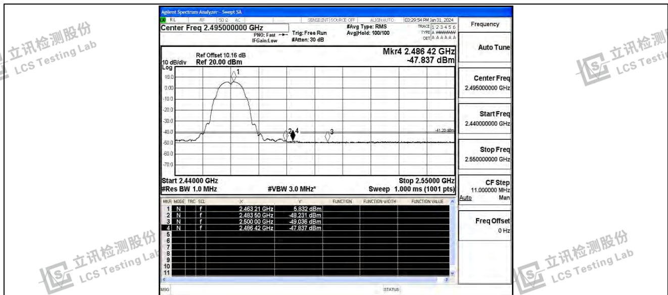
11B_Ant_High_2462_Peak
