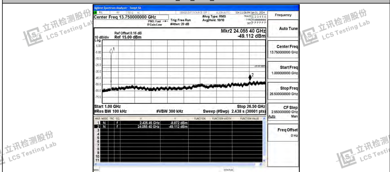
11N40SISO_Ant_2422_1000~26500
