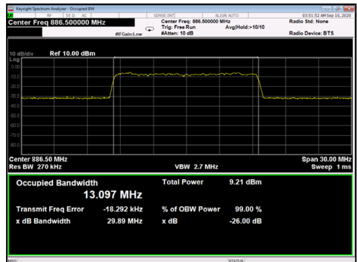
Figure 283: 256QAM 15MHz B.W.; 886.5MHz, 60kHz - Input
