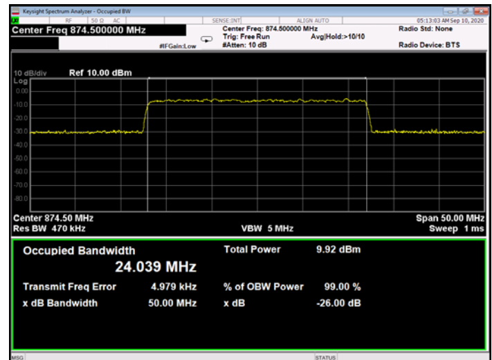
Figure 293: 256QAM 25MHz B.W.; 874.5MHz, 15kHz - Input
