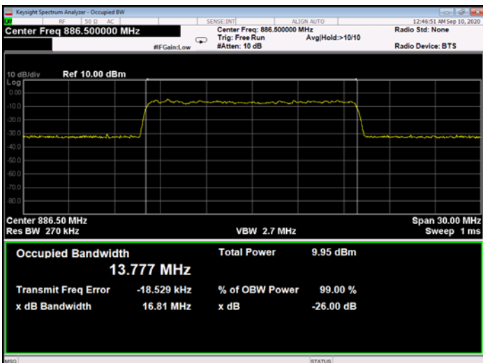
Figure 324: QPSK 15MHz B.W.; 886.5MHz, 30kHz - Input
