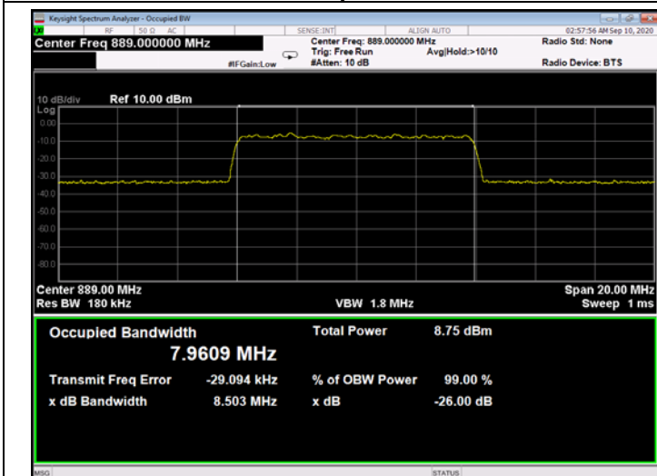
Figure 274: 256QAM 10MHz B.W.; 889.0MHz, 60kHz - Input
