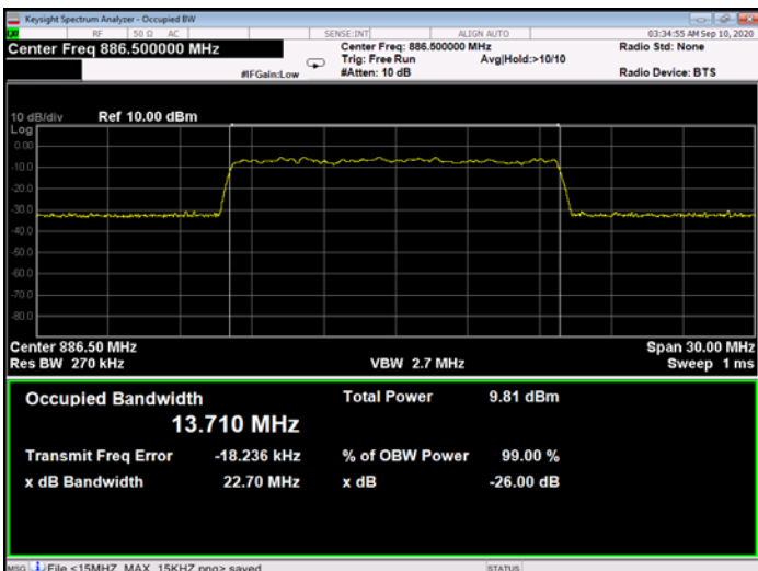
Figure 282: 256QAM 15MHz B.W.; 886.5MHz, 30kHz - Input
