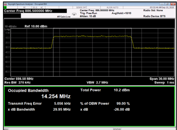
Figure 281: 256QAM 15MHz B.W.; 886.5MHz, 15kHz - Input
