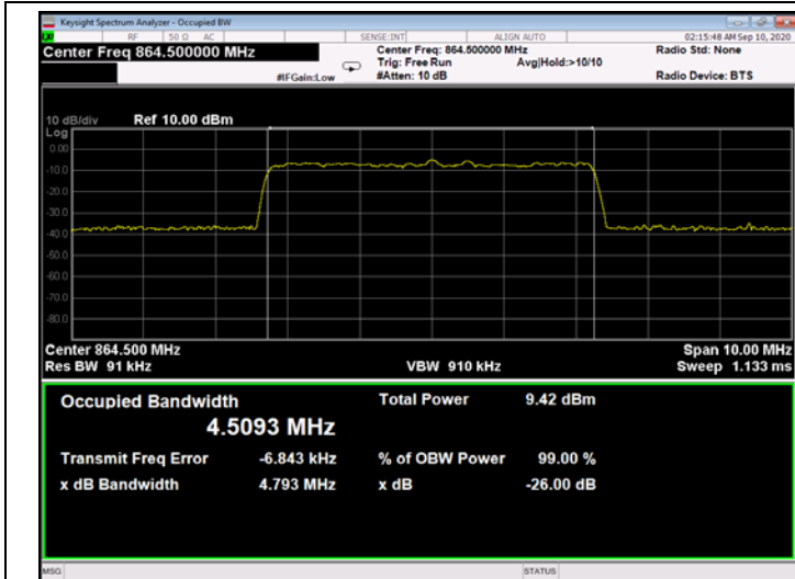
Figure 260: 256QAM 5MHz B.W.; 864.5MHz, 15kHz - Input
