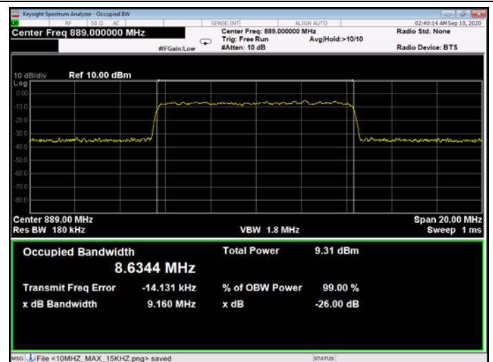
Figure 273: 256QAM 10MHz B.W.; 889.0MHz, 30kHz - Input
