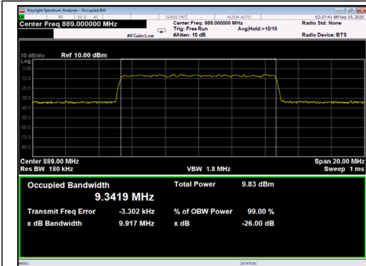
Figure 272: 256QAM 10MHz B.W.; 889.0MHz, 15kHz - Input
