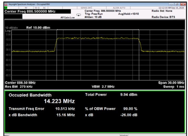
Figure 323: QPSK 15MHz B.W.; 886.5MHz, 15kHz - Input
