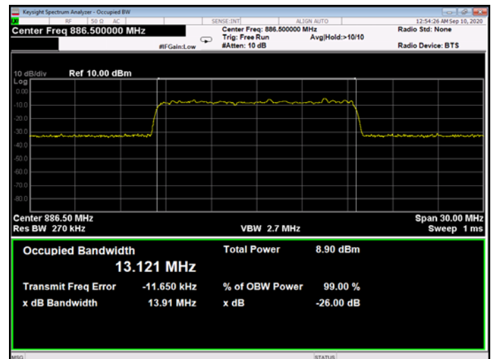
Figure 325: QPSK 15MHz B.W.; 886.5MHz, 60kHz - Input
