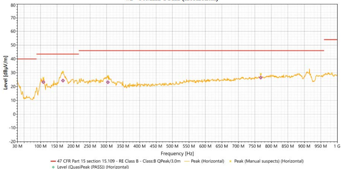
#2 - 30MHz-1GHz (Horizontal)
