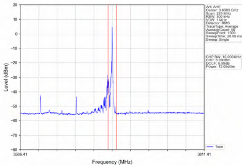
n78d_30kHz_SISO_NTNV_90MHz_CP-OFDM QPSK_3654.99MHz_Edge_1RB_Right
