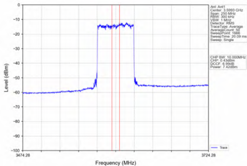
n78d_30kHz_SISO_NTNV_100MHz_DFT-s-OFDM_64_QAM_3600MHz_Inner_Full
