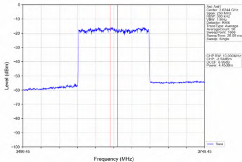
n78d_30kHz_SISO_NTNV_100MHz_DFT-s-OFDM_QPSK_3624.99MHz_Inner_Full
