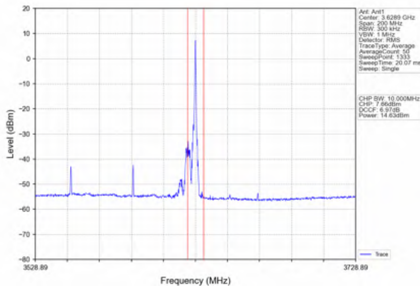
n78d_30kHz_SISO_NTV_80MHz_CP-OFDM QPSK_3590.01MHz_Edge_1RB_Right
