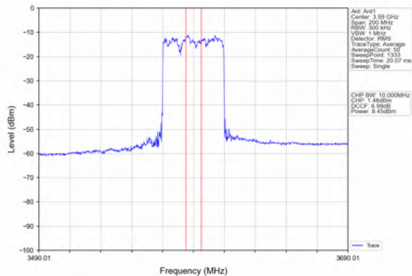
n78d_30kHz_SISO_NTNV_80MHz_CP-OFDM 64 QAM_3590.01MHz_Inner_Full
