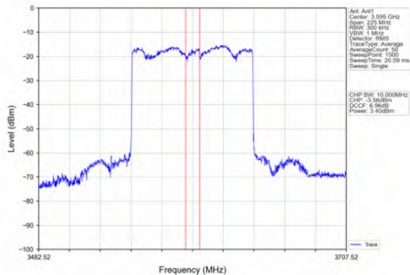
n78d_30kHz_SISO_NTNV_90MHz_CP-OFDM_256_QAM_3595.02MHz_Inner_Full
