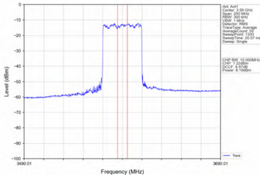
n78d_30kHz_SISO_NTNV_80MHz_CP-OFDM_QPSK_3590.01MHz_Inner_Full
