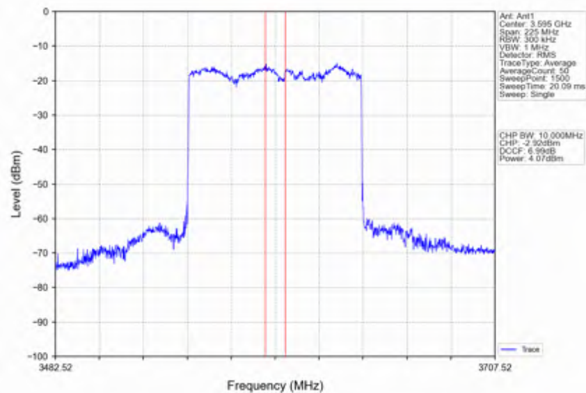
n78d_30kHz_SISO_NTNV_90MHz_CP-OFDM 16 QAM_3595.02MHz_Inner_Full
