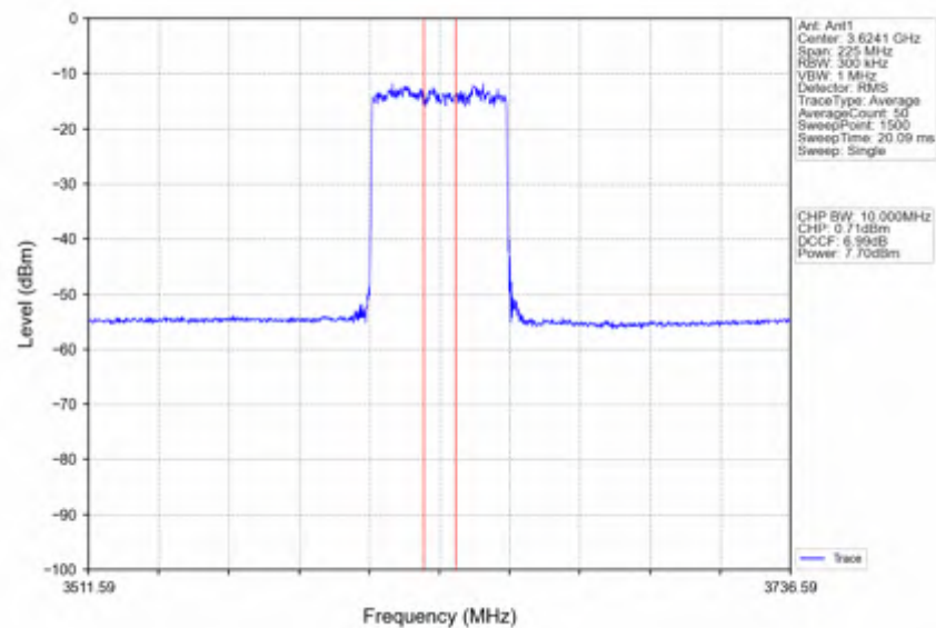
n78d_30kHz_SISO_NTNV_90MHz_DFT-s-OFDM 16 QAM_3624.99MHz_Inner_Full
