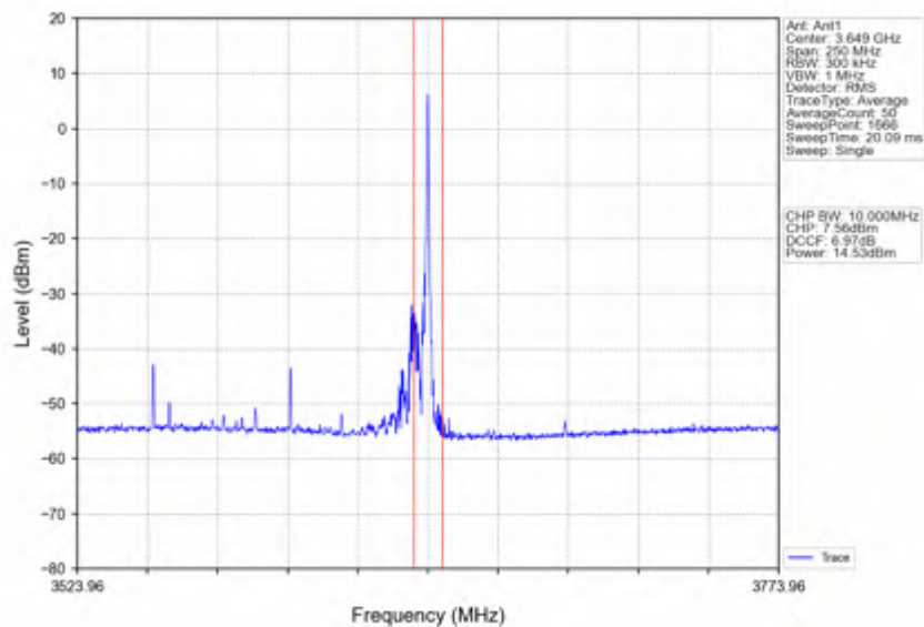
n78d_30kHz_SISO_NTNV_100MHz_DFT-s-OFDM QPSK_3600MHz_Edge_1RB_Right
