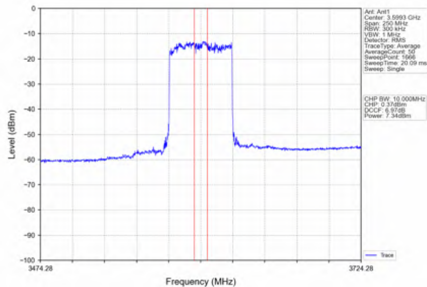
n78d_30kHz_SISO_NTNV_100MHz_DFT-s-OFDM QPSK_3600MHz_Inner_Full
