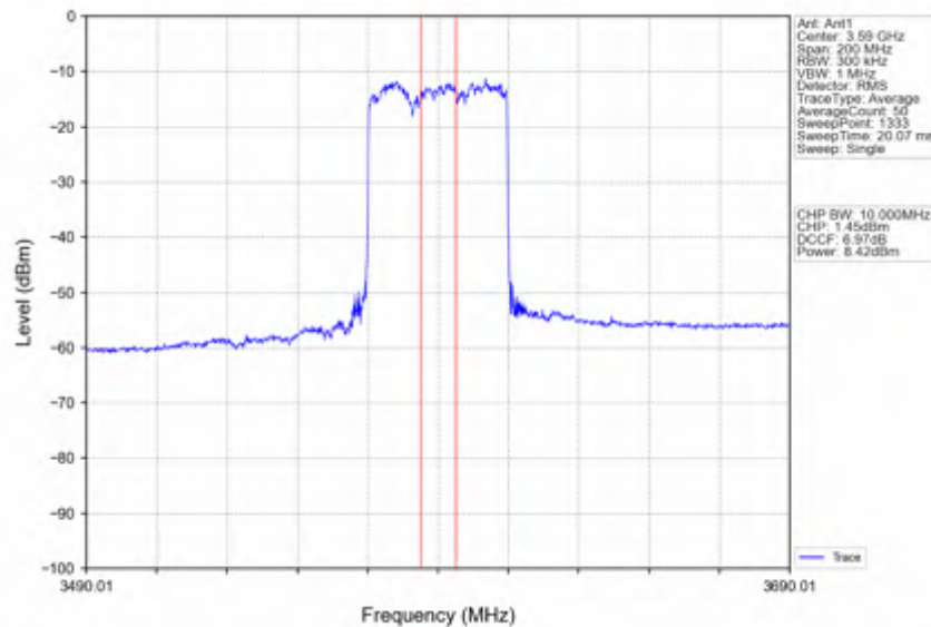
n78d_30kHz_SISO_NTNV_80MHz_CP-OFDM_256_QAM_3590.01MHz_Inner_Full
