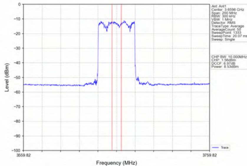
n78d_30kHz_SISO_NTNV_80MHz_DFT-s-OFDM 64 QAM_3660MHz_Inner_Full
