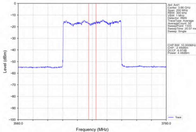
n78d_30kHz_SISO_NTNV_80MHz_CP-OFDM_256_QAM_3660MHz_Inner_Full
