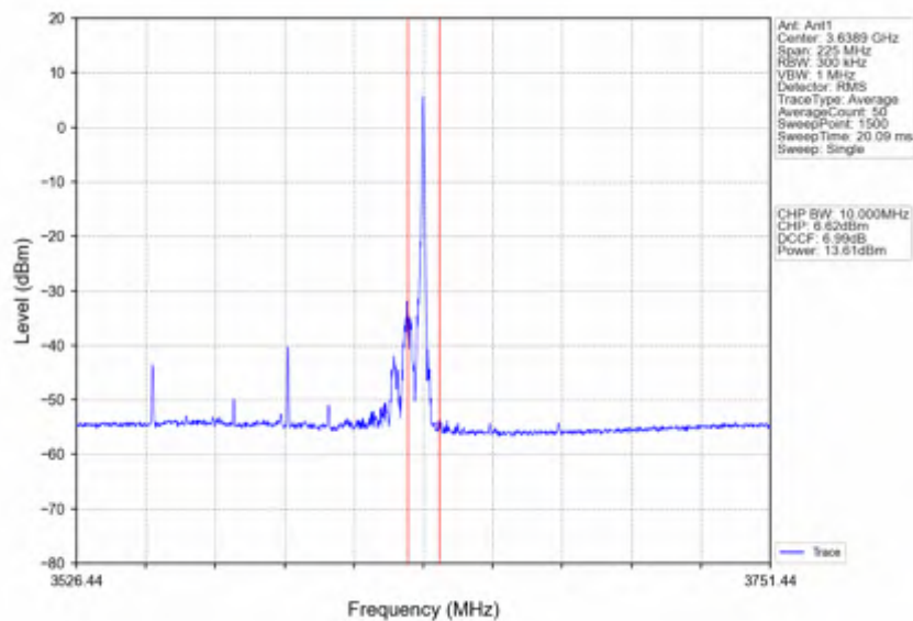
n78d_30kHz_SISO_NTNV_90MHz_DFT-s-OFDM 64 QAM_3595.02MHz_Edge_1RB_Right
