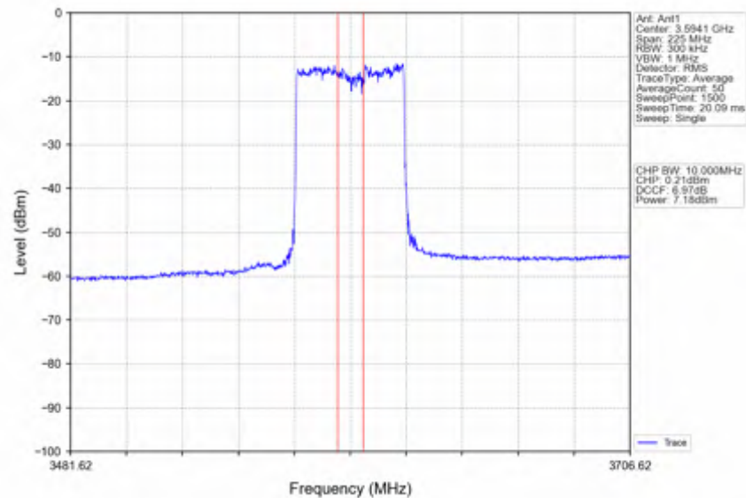
n78d_30kHz_SISO_NTNV_90MHz_DFT-s-OFDM_256_QAM_3595.02MHz_Inner_Full
