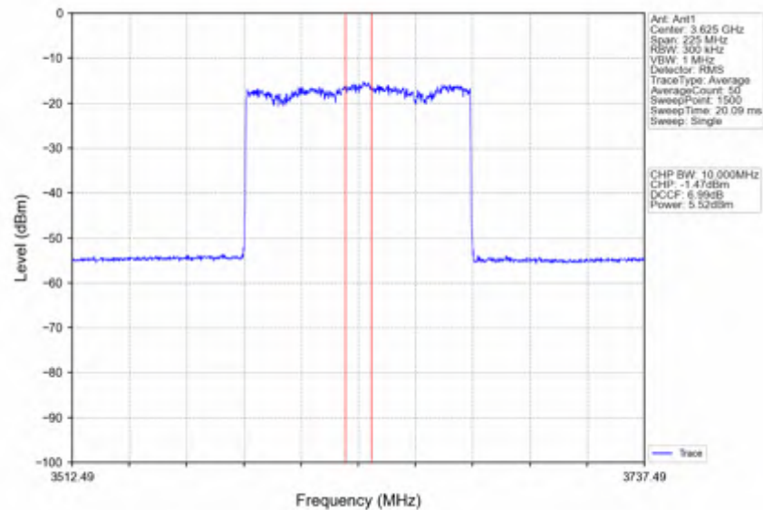
n78d_30kHz_SISO_NTNV_90MHz_CP-OFDM 64 QAM_3624.99MHz_Inner_Full
