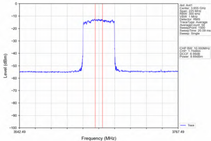
n78d_30kHz_SISO_NTNV_90MHz_CP-OFDM_256_QAM_3654.99MHz_Inner_Full
