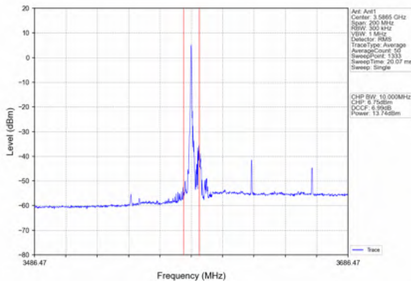
n78d_30kHz_SISO_NTV_80MHz_CP-OFDM QPSK_3624.99MHz_Inner_1RB_Right
