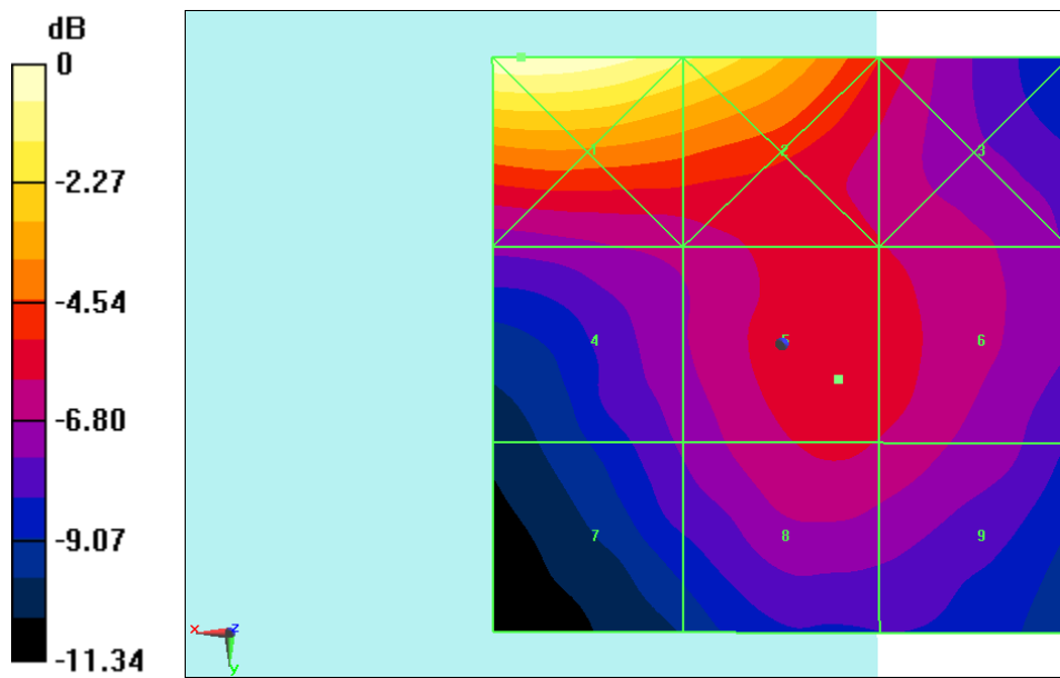
Fig B.1 HAC RF E-Field LTE Band43 QPSK
