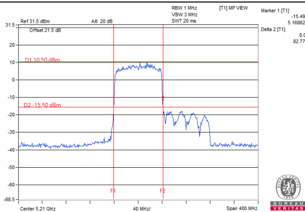
802.11ax (HE80+80)_Chain 1 / CH42
