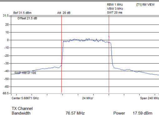
802.11ax (HE80)_Chain 1 / CH138 (U-NII-2C Band)
