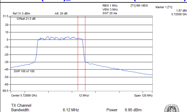
802.11ax (HE40)_Chain 2 / CH142 (U-NII-3 Band)
