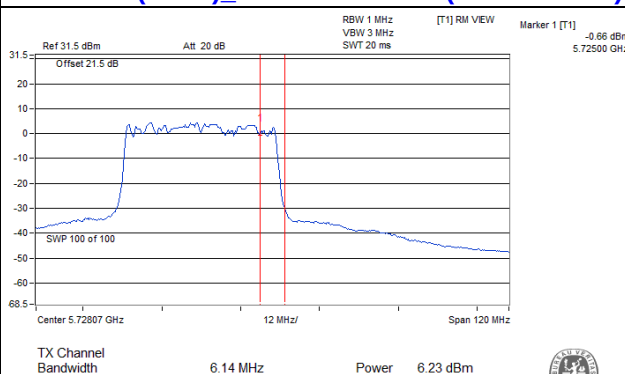
802.11ax (HE40)_Chain 1 / CH142 (U-NII-3 Band)
