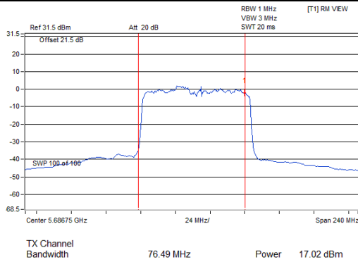
802.11ax (HE80)_Chain 0 / CH138 (U-NII-2C Band)
