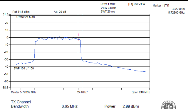
802.11ax (HE80)_Chain 2 / CH138 (U-NII-3 Band)
