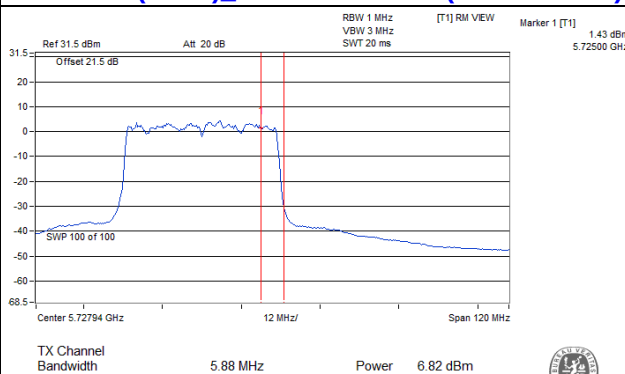
802.11ax (HE40)_Chain 0 / CH142 (U-NII-3 Band)
