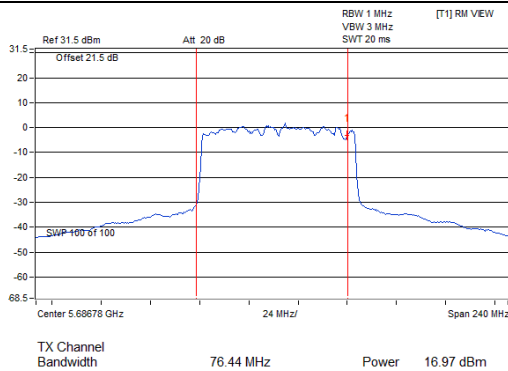
802.11ax (HE80)_Chain 2 / CH138 (U-NII-2C Band)
