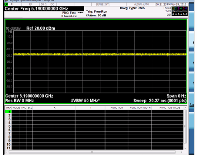
11AC40MIMO -5190
