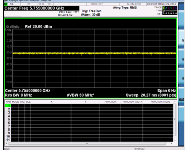
11AC40MIMO -5755
