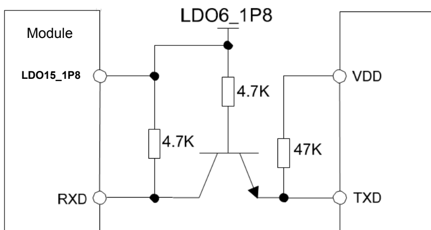
Figure 22 RX Connection Diagram
