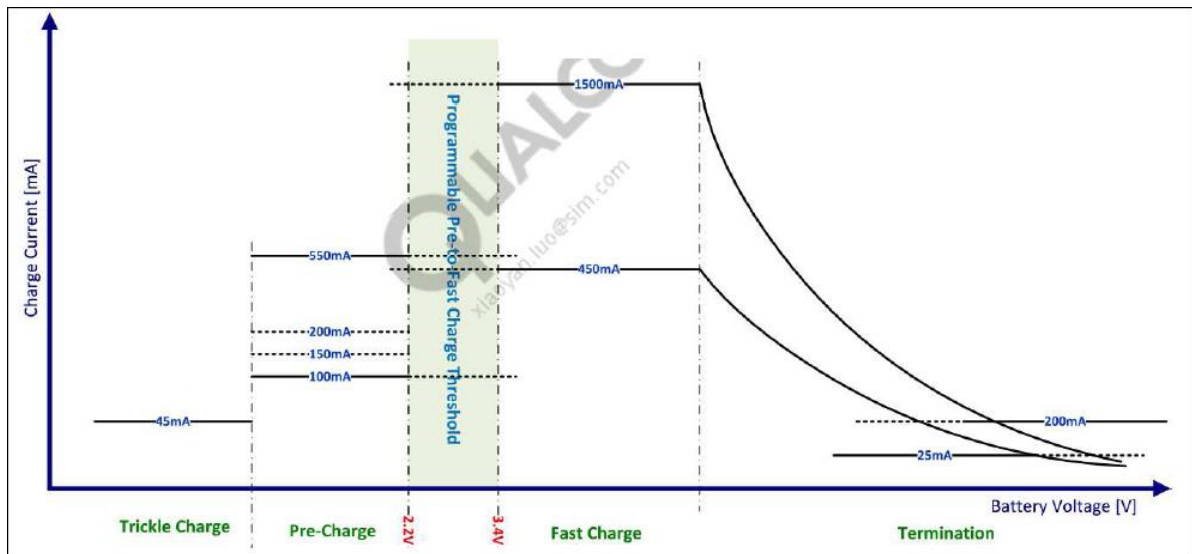
Figure 33 Charging diagram
