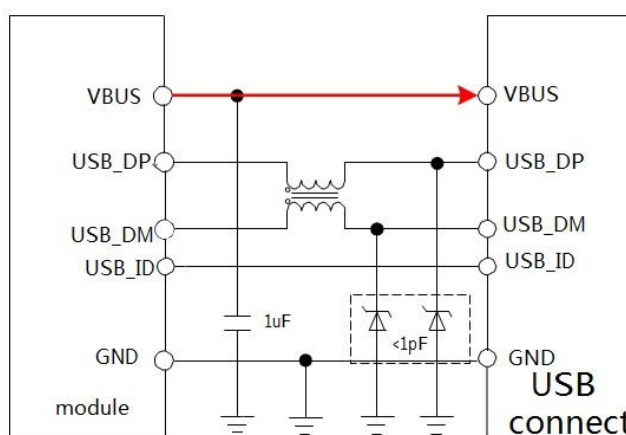
Figure 32 USB-OTG Connection Diagram
