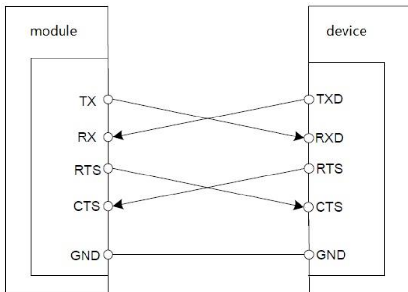
Figure 20 Serial Port Connection Diagram
