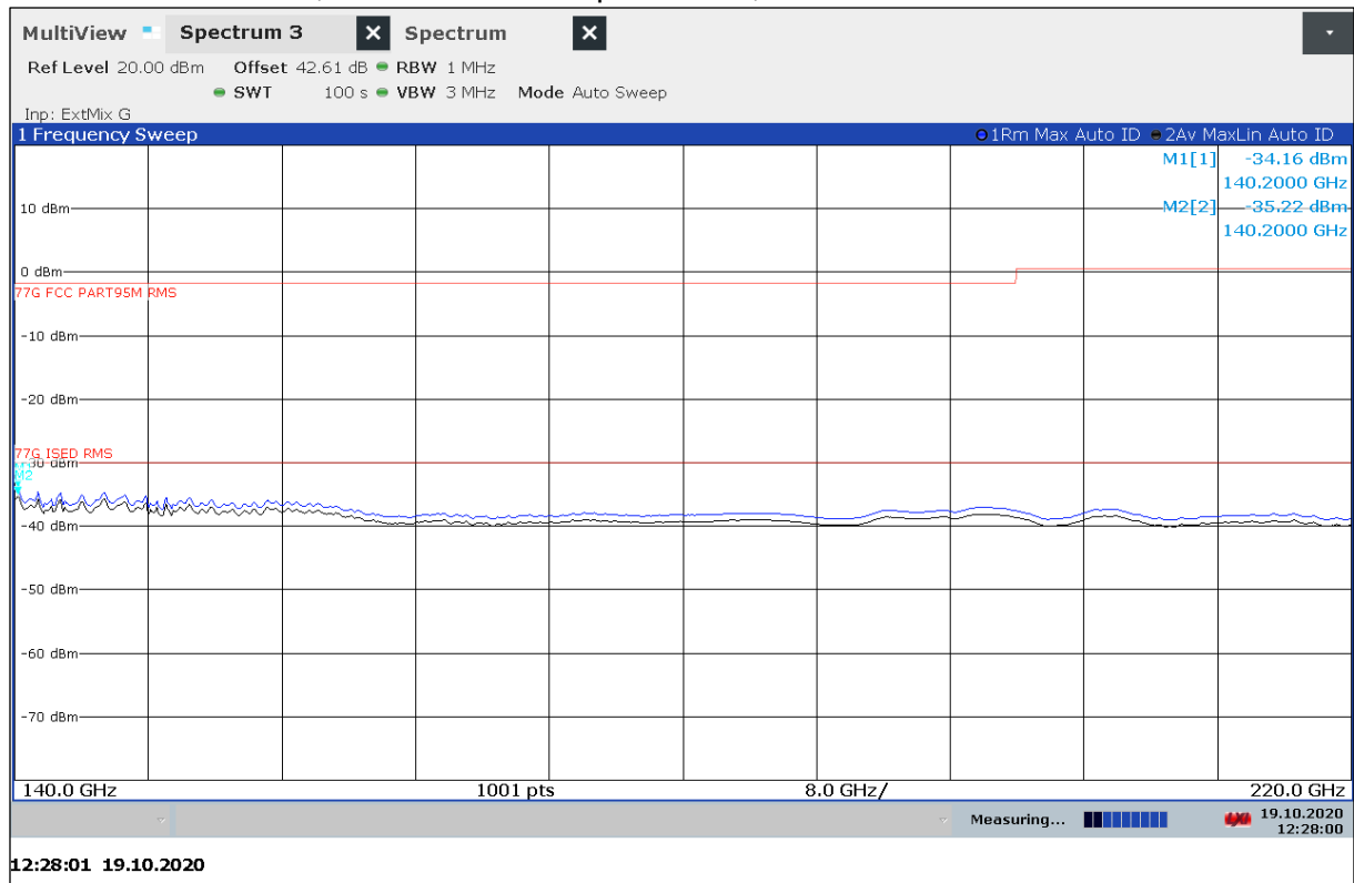
Plot 39: 140 GHz – 220 GHz, vertical / horizontal polarization, Mode 3 and Mode 6
