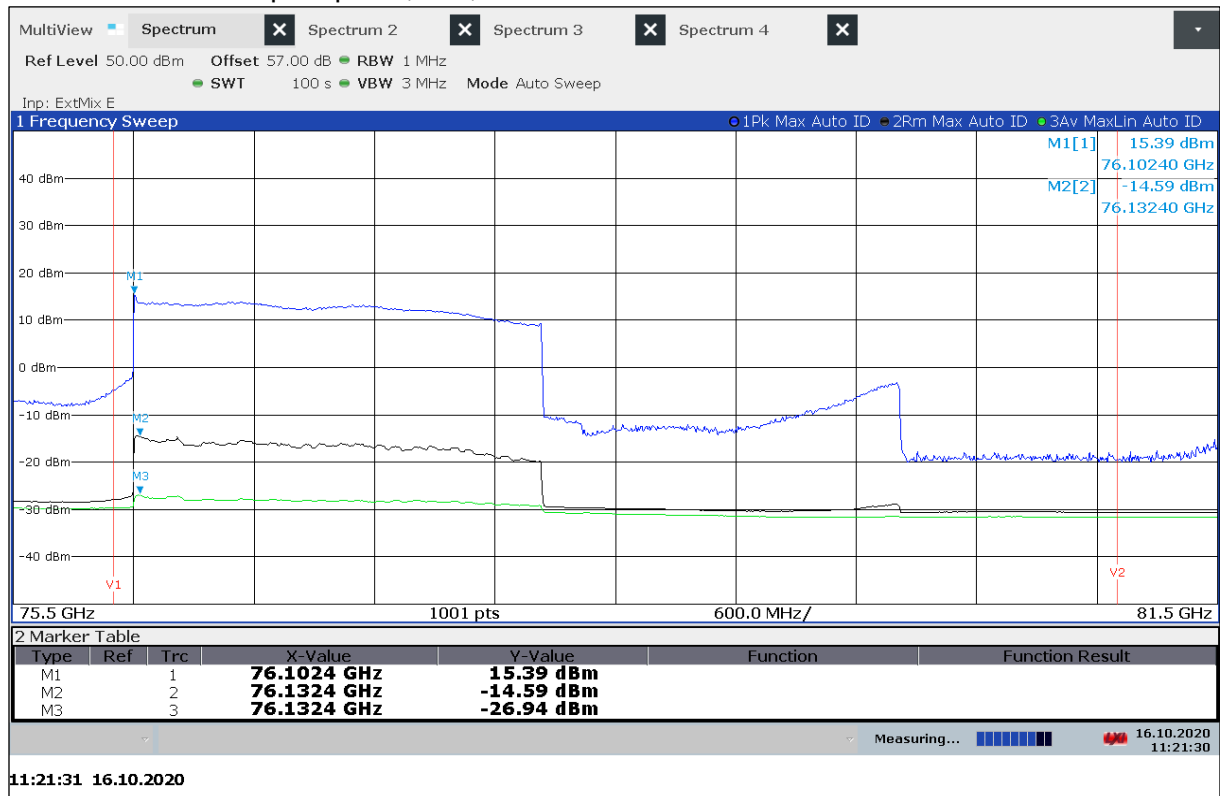
Plot 6: Mode 6 – Radiated peak power, PSD, T_{\max} / V_{\text{nom}}
