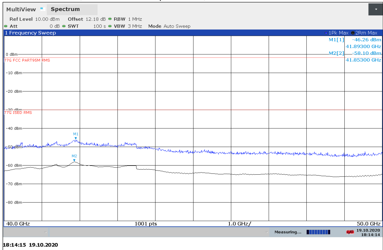
Plot 33: 40 GHz – 50 GHz, vertical / horizontal polarization, Mode 3 and Mode 6
