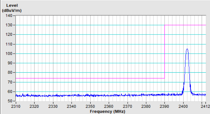
BT GFSK Channel 0
