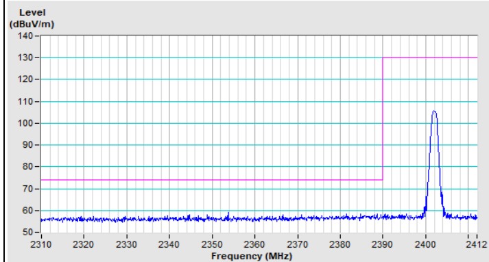
BT GFSK Channel 0
