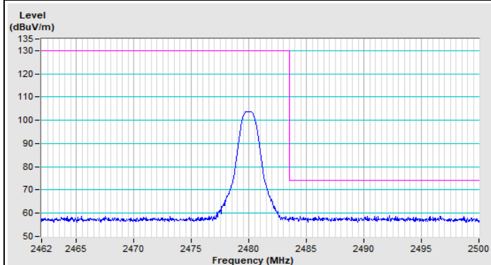
BT GFSK Channel 78
