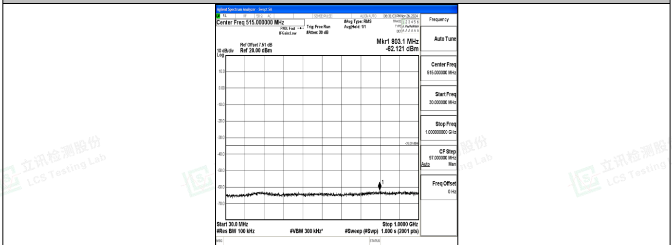
Band7_20MHz_QPSK_21100_1RB#0_30~1000_30~1000
