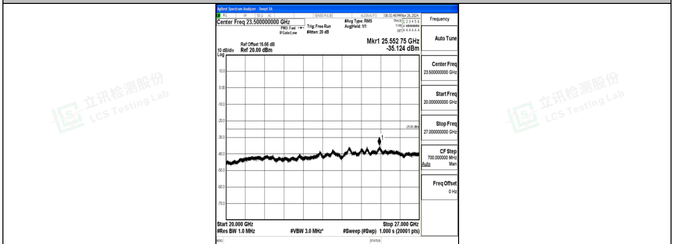
Band7_20MHz_16QAM_21100_1RB#0_20000~27000_20000~27000
