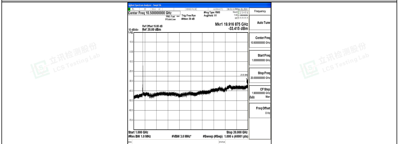
Band7_20MHz_QPSK_21100_1RB#0_1000~20000_1000~20000
