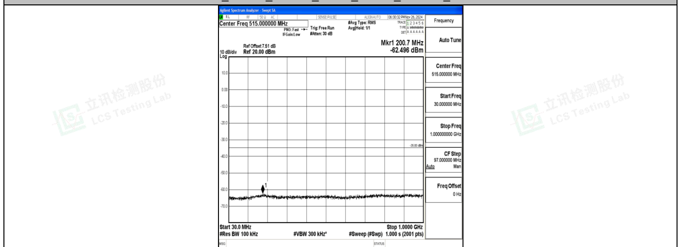
Band7_20MHz_16QAM_20850_1RB#0_30~1000_30~1000
