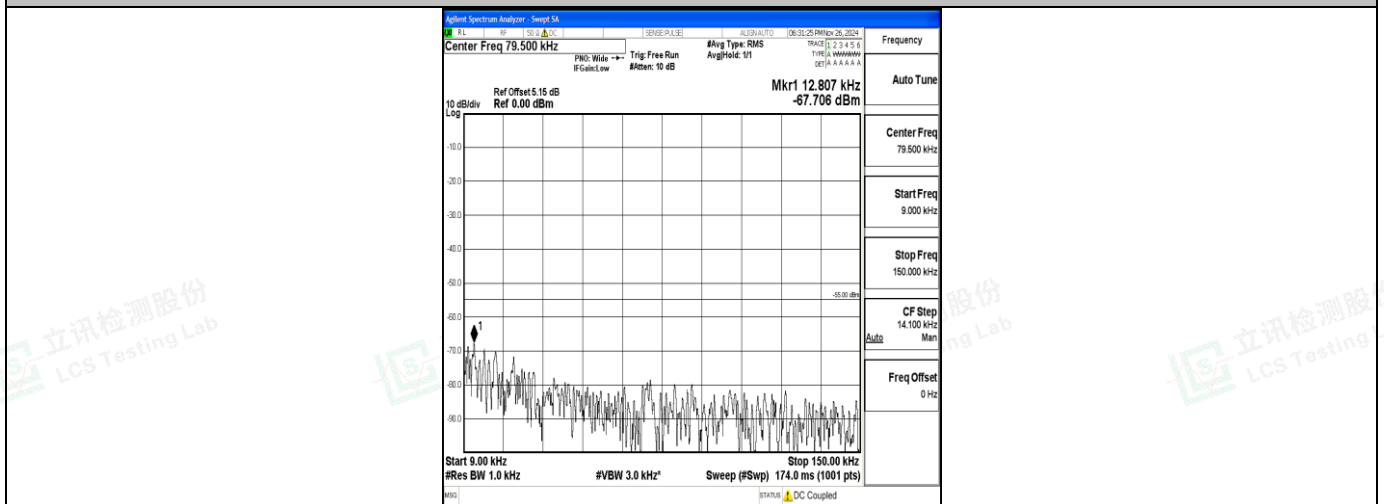
Band7_20MHz_16QAM_21100_1RB#0_0.009~0.15_0.009~0.15
