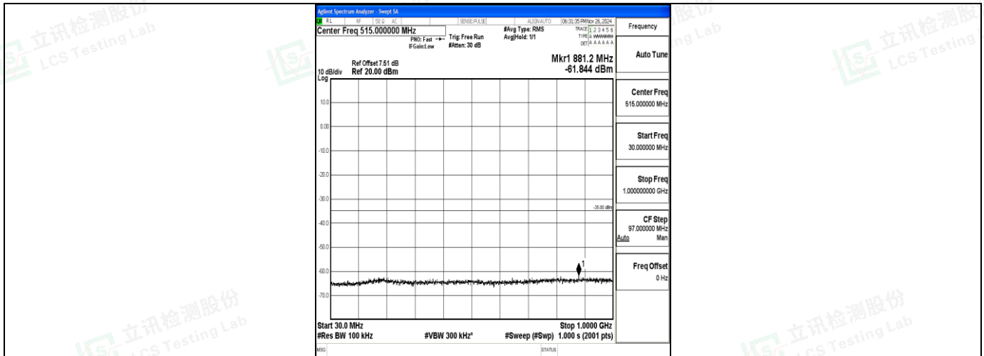
Band7_20MHz_16QAM_21100_1RB#0_30~1000_30~1000
