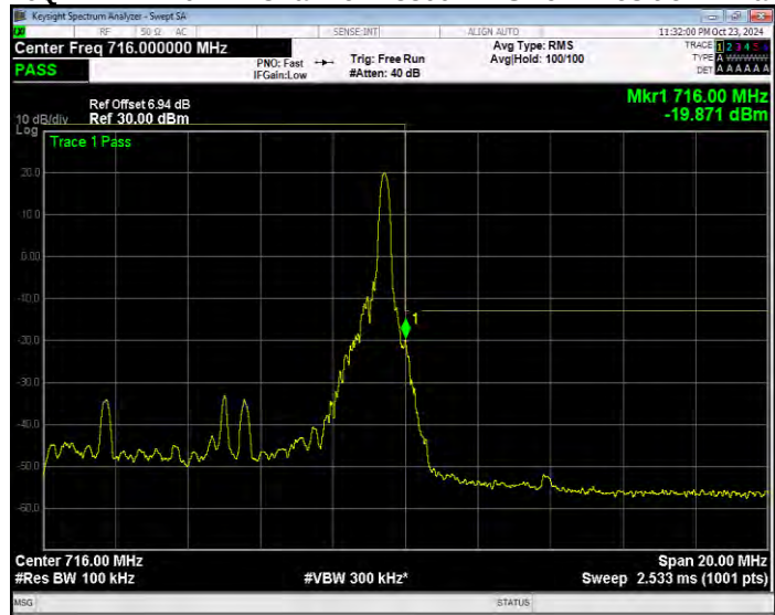
Band17 16QAM BW=10MHz Channel=23800 RB Size=50 Position=#0 Extended
