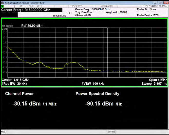
Band25 16QAM BW=1.4MHz Channel=26683 RB Size=1 Position=#0 Normal
