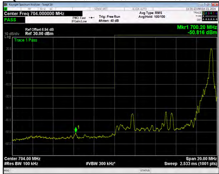
Band17 16QAM BW=10MHz Channel=23780 RB Size=50 Position=#0 Extended
