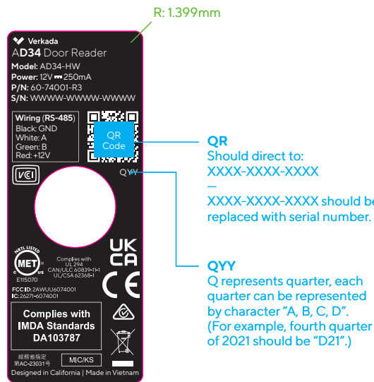
AD34-HW Door Reader Product Label - PVT V1 25.3 x 65.8 mm
