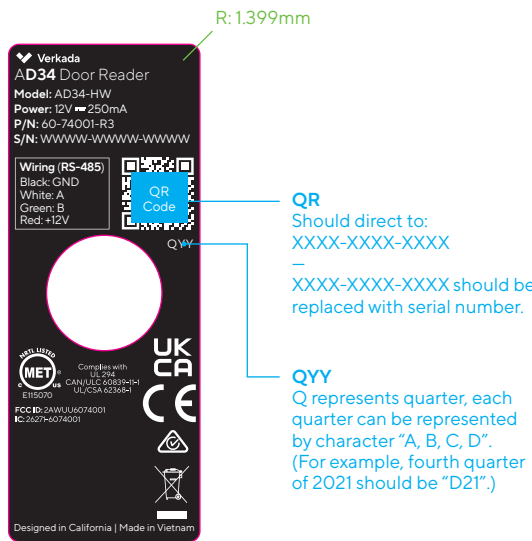
AD34-HW Door Reader Product Label - PVT V2 25.3 x 65.8 mm
