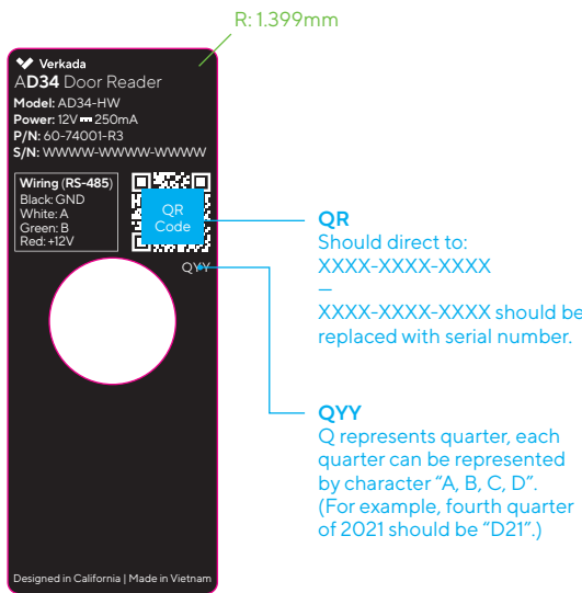
AD34-HW Door Reader Product Label - PVT V3 25.3 x 65.8 mm
