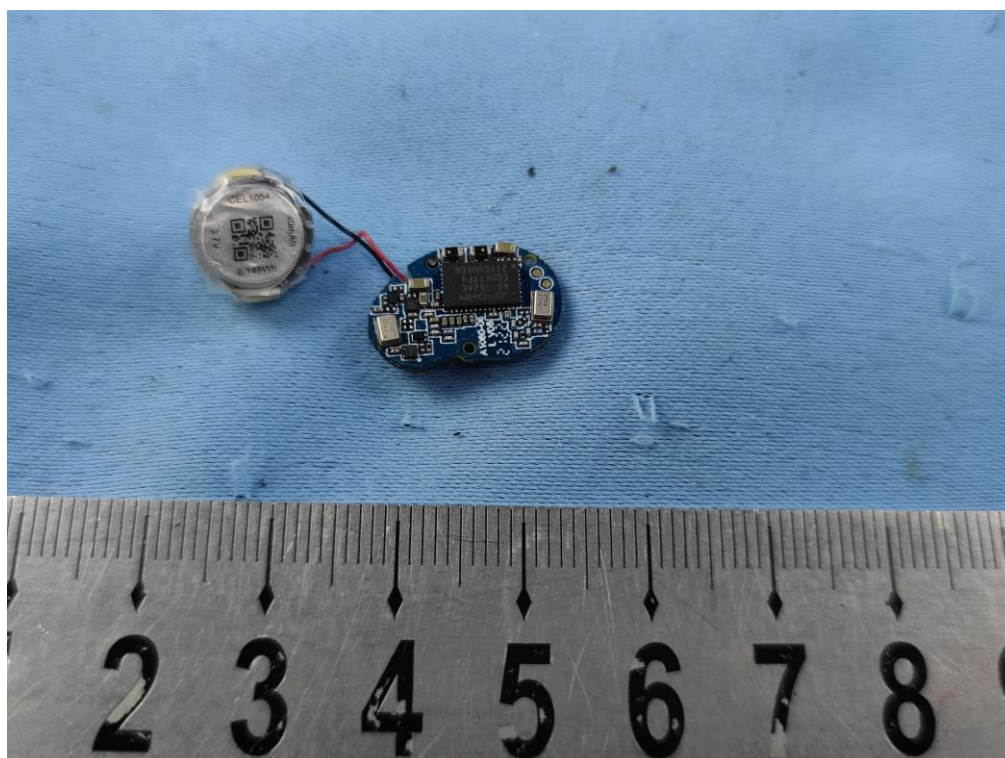
Left earbud
