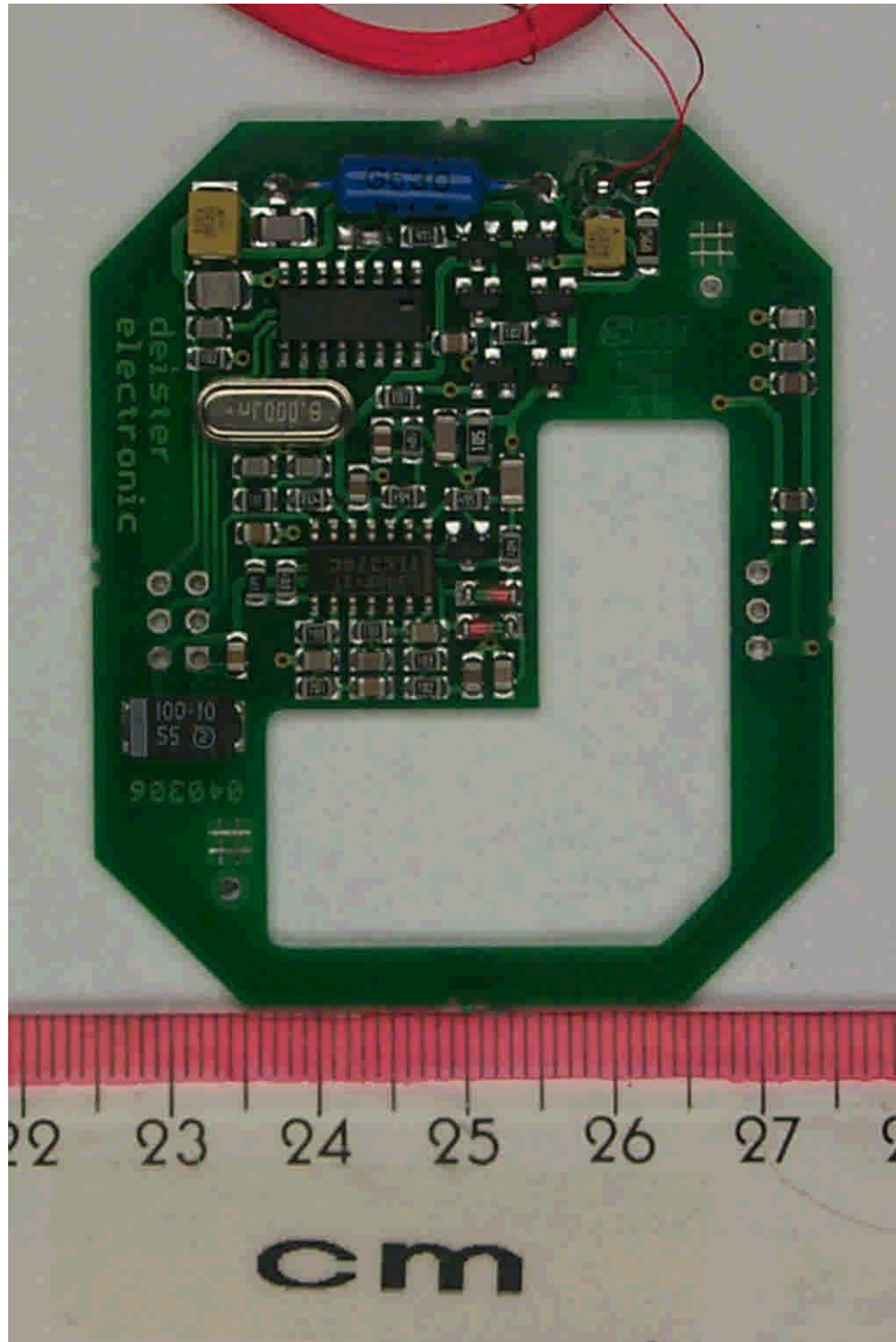
41092C_a.jpg KPD5 / SWH-4200, antenna PCB, top view
