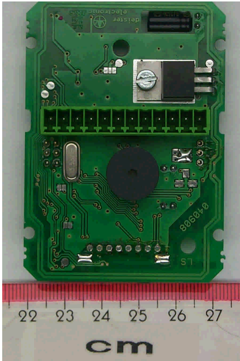
41092C_b.jpg KPD5 / SWH-4200, main PCB, top view
