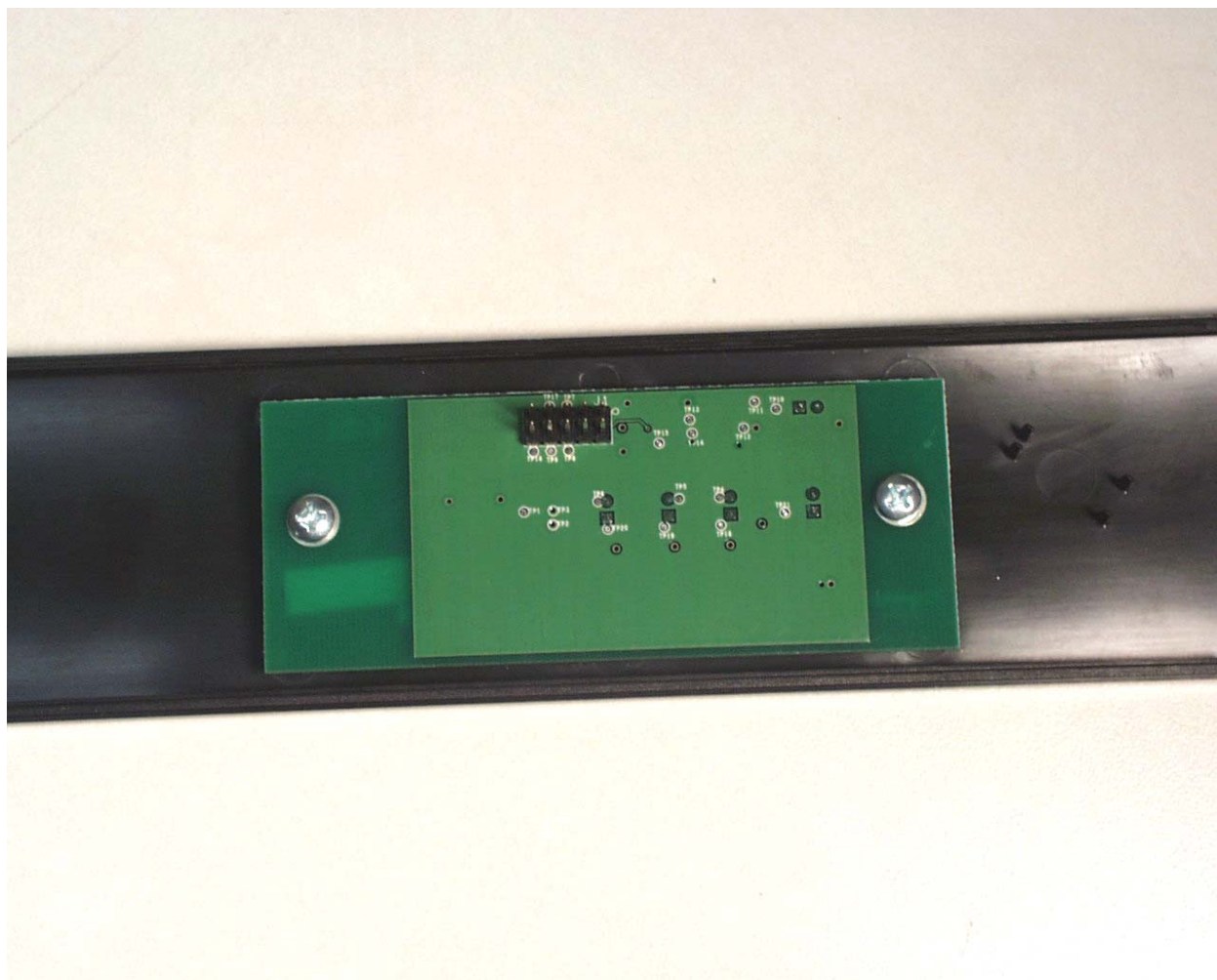
Photograph 11 - Rear View of the Front Panel PCB
