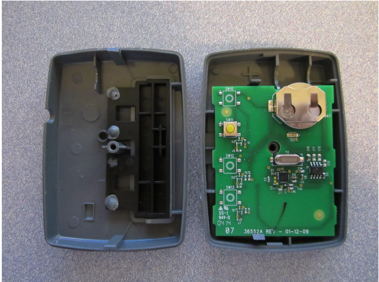
Figure 3: OCDFX1 Internal View / PCB Top
