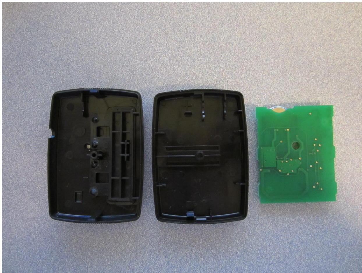
Figure 2: GIDFX1 Internal View / PCB Bottom
