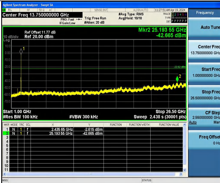
11N20SISO-Ant1-2437-1000~26500-PASS
