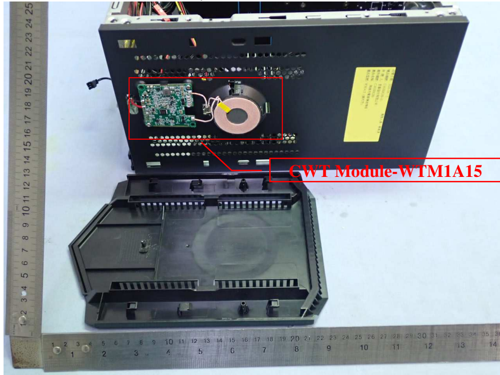
Figure 11 Personal Computer D19W6, Internal View (Removed Cover)
