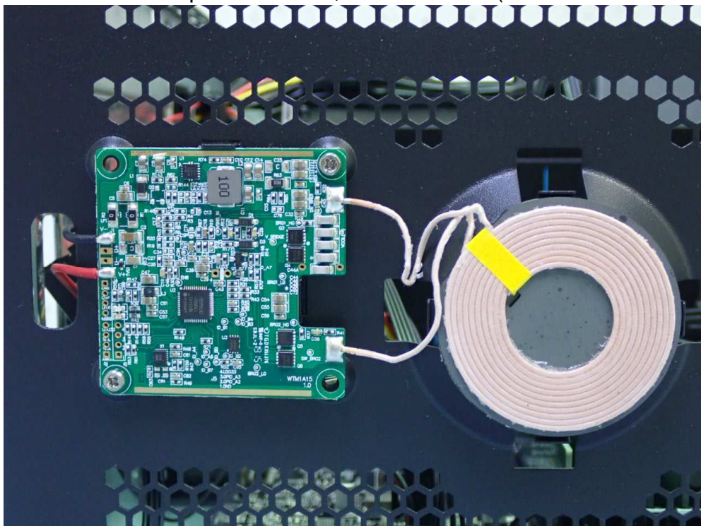
Figure 12 Personal Computer D19W6, Internal View (CWT Module-WTM1A15)
