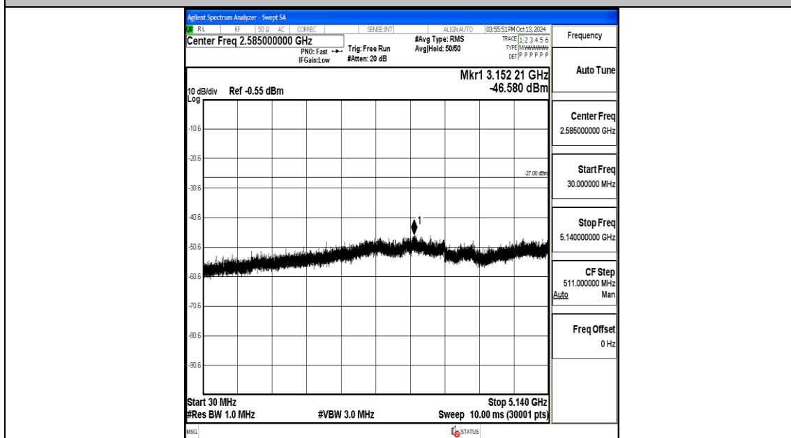
11AC80MIMO-Ant1-5210-30~5140-PASS
