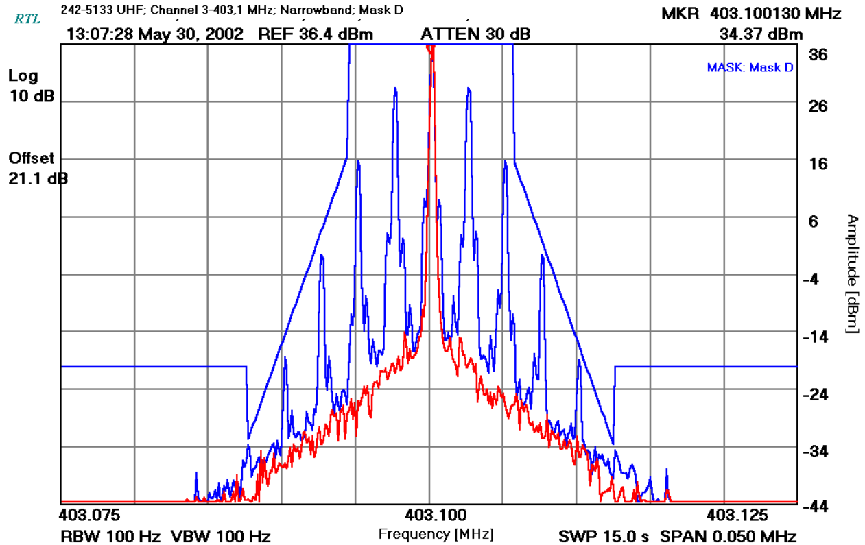
PLOT 8-1: MASK D (403.1 MHz; CH3; NARROWBAND)
