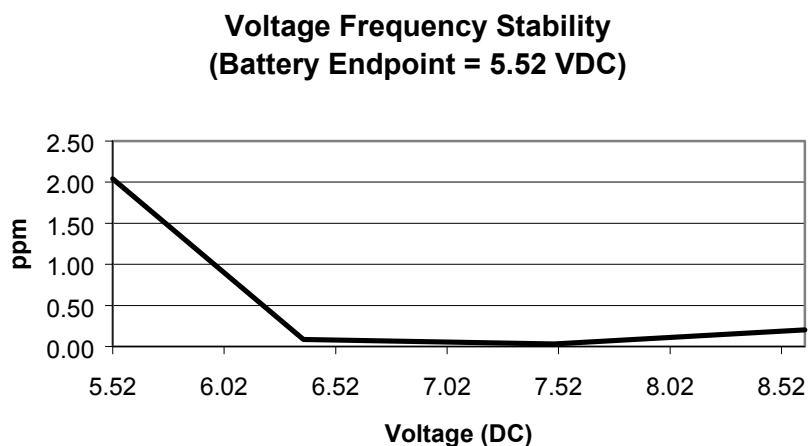
PLOT 11-2: VOLTAGE FREQUENCY STABILITY - §2.1055
