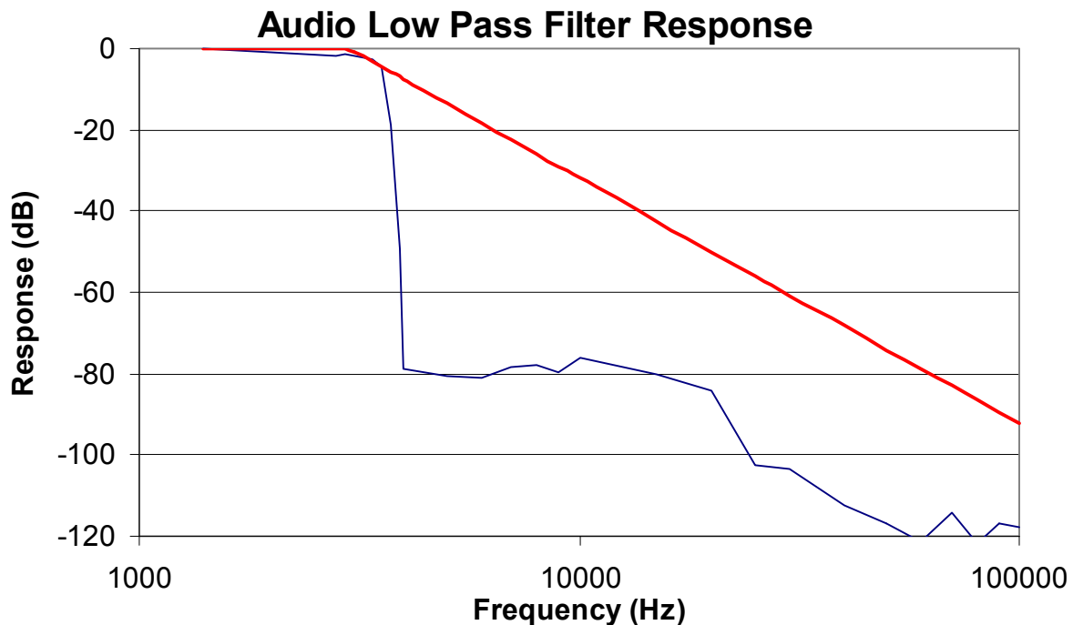
PLOT 6-1: AUDIO LOW PASS FILTER RESPONSE (CHANNEL 3)
