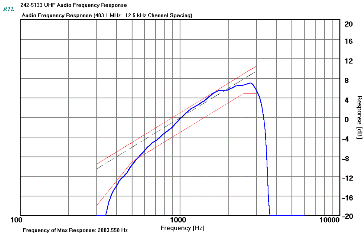
PLOT 5-1: AUDIO FREQUENCY RESPONSE CHANNEL 3 AT 403.1 MHZ
