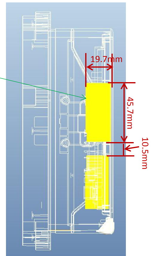
WIFI Antenna
