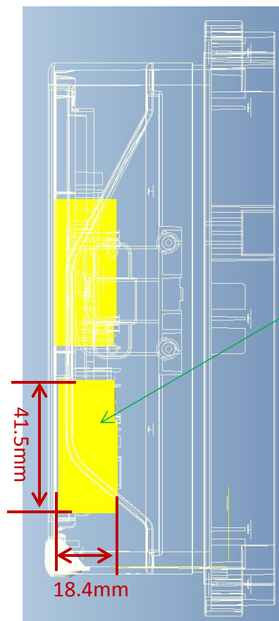
4G Diversity Antenna
