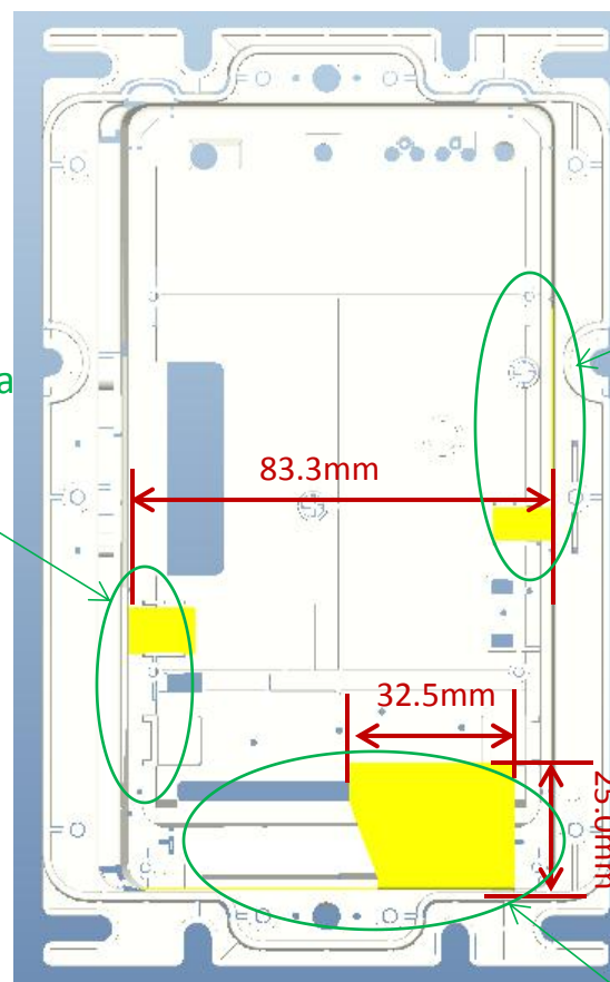
WIFI Antenna
