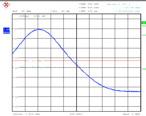
Band25-10MHz-16QAM-26640-1RB#49
