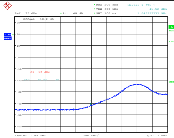
Band25-10MHz-16QAM-26090-1RB#49
