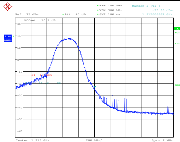
Band25-5MHz-16QAM-26665-1RB#24
