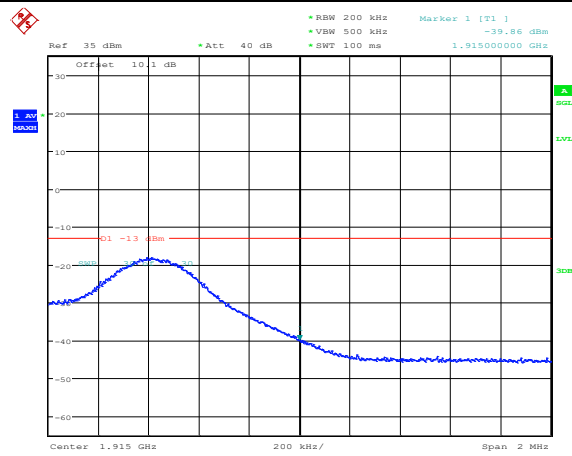
Band25-10MHz-16QAM-26640-1RB#0
