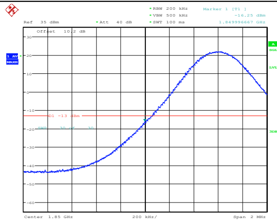
Band25-10MHz-QPSK-26090-1RB#0
