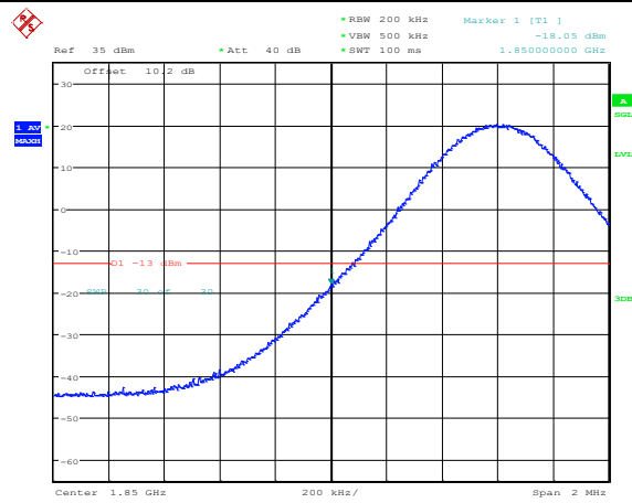
Band25-10MHz-16QAM-26090-1RB#0
