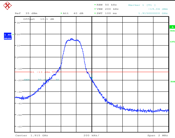
Band25-3MHz-16QAM-26675-1RB#14
