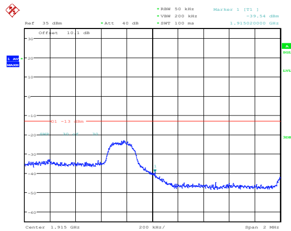
Band25-3MHz-16QAM-26675-1RB#0
