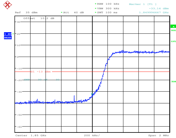
Band25-5MHz-QPSK-26665-1RB#0
