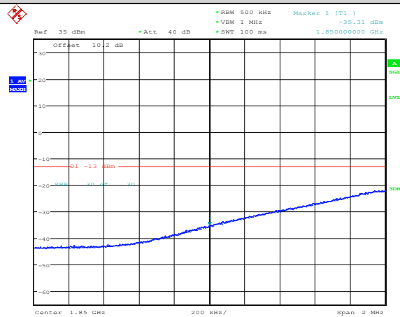
Band25-20MHz-16QAM-26140-1RB#99
