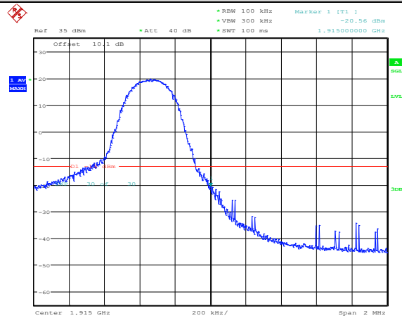
Band25-5MHz-QPSK-26665-1RB#24
