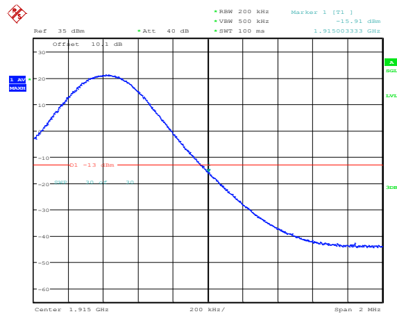
Band25-10MHz-QPSK-26640-1RB#49
