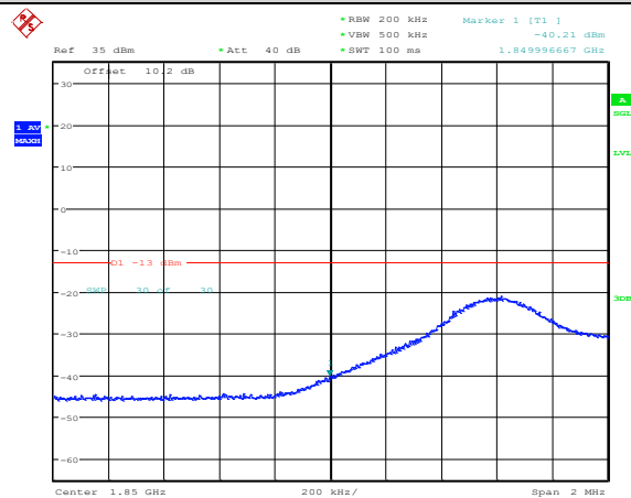
Band25-10MHz-QPSK-26090-1RB#49
