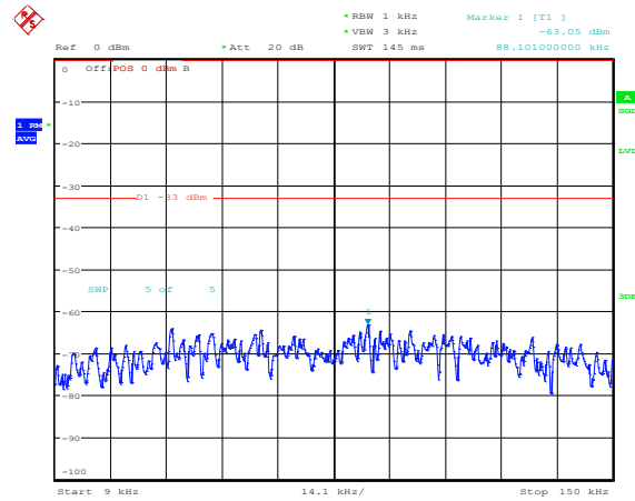
Band25-1.4MHz-QPSK-26047-1RB#0-Range1:0.009~0.15MHz
