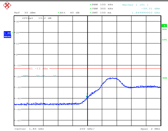
Band25-5MHz-QPSK-26065-1RB#24
