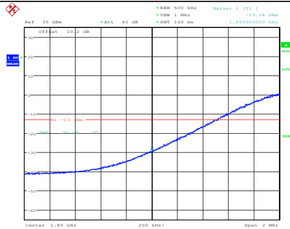
Band25-20MHz-QPSK-26140-100RB#0
