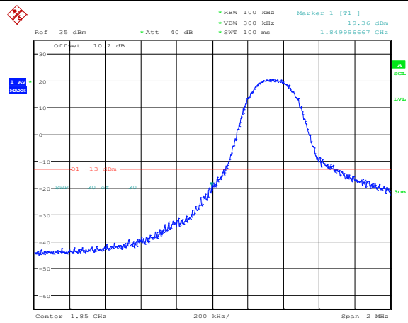
Band25-5MHz-QPSK-26065-1RB#0
