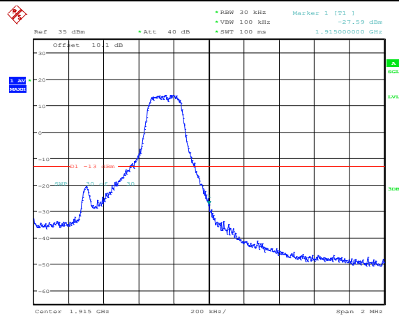
Band25-1.4MHz-16QAM-26683-1RB#5
