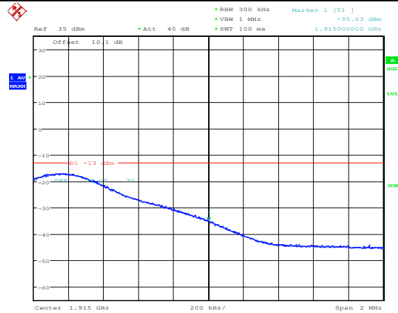
Band25-15MHz-QPSK-26615-1RB#0
