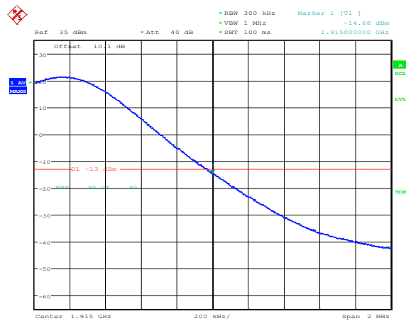
Band25-15MHz-QPSK-26615-1RB#74
