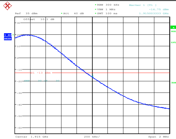
Band25-15MHz-16QAM-26615-1RB#74
