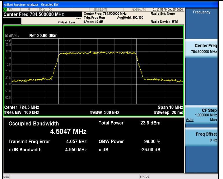
Band13-5MHz-16QAM-23255-25RB#0-PASS
