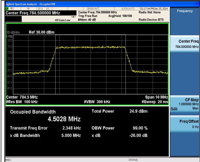
Band13-5MHz-QPSK-23255-25RB#0-PASS
