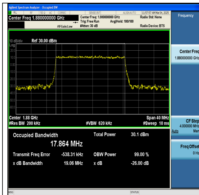
NTNV-n2-PC3-15-20-M-DFT-16QAM-Outer_Full-Ant1- PASS
