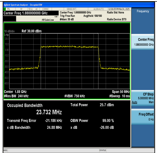
NTNV-n2-PC3-15-25-M-CP-256QAM-Outer_Full-Ant1- PASS
