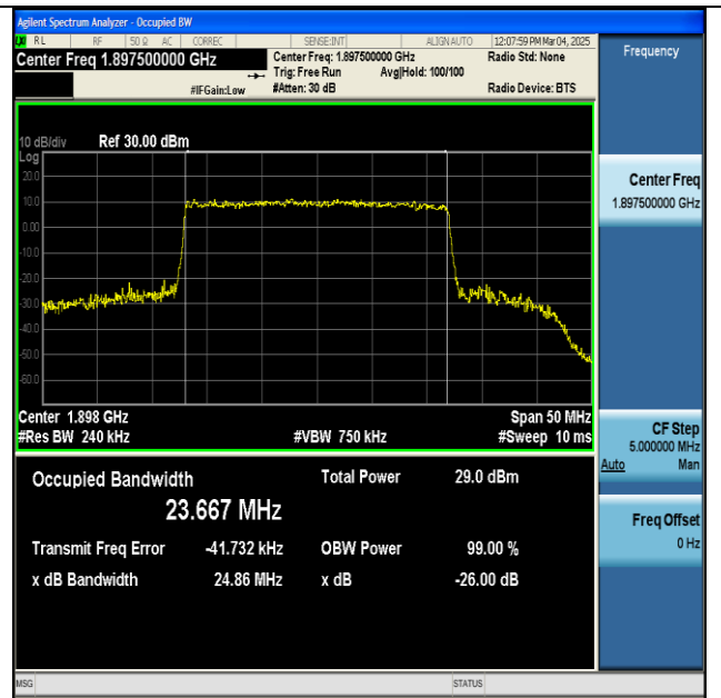
NTNV-n2-PC3-15-25-H-CP-64QAM-Outer_Full-Ant1-PASS
