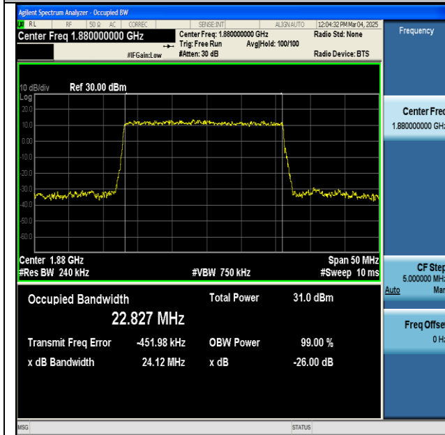
NTNV-n2-PC3-15-25-M-DFT-QPSK-Outer_Full-Ant1-PASS
