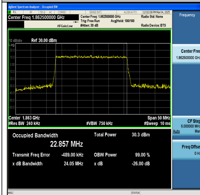
NTNV-n2-PC3-15-25-L-DFT-16QAM-Outer_Full-Ant1- PASS
