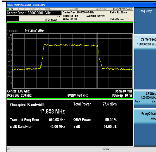
NTNV-n2-PC3-15-20-M-DFT-256QAM-Outer_Full-Ant1- PASS
