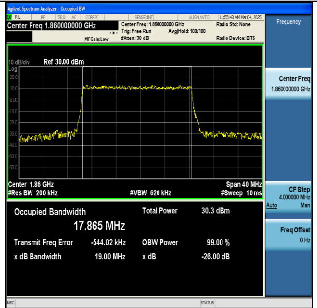
NTNV-n2-PC3-15-20-L-DFT-16QAM-Outer_Full-Ant1-PASS
