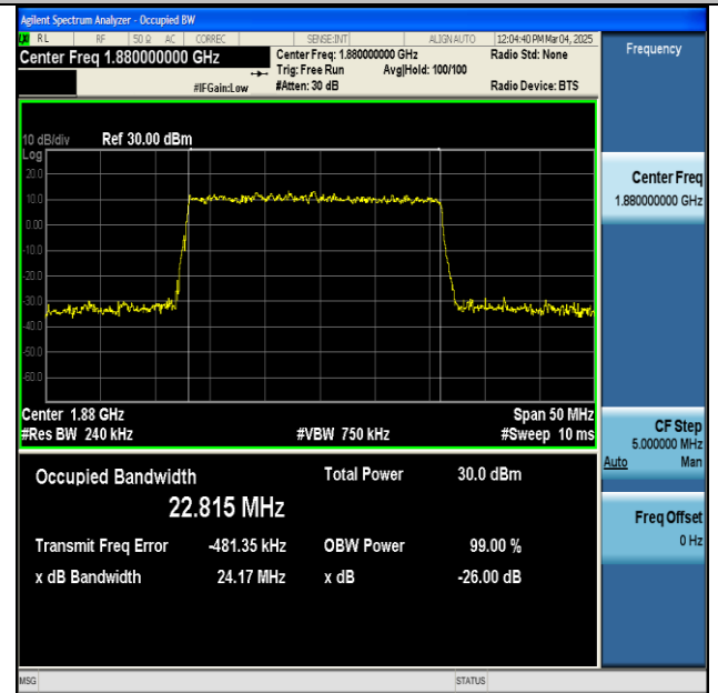
NTNV-n2-PC3-15-25-M-DFT-16QAM-Outer_Full-Ant1-PASS
