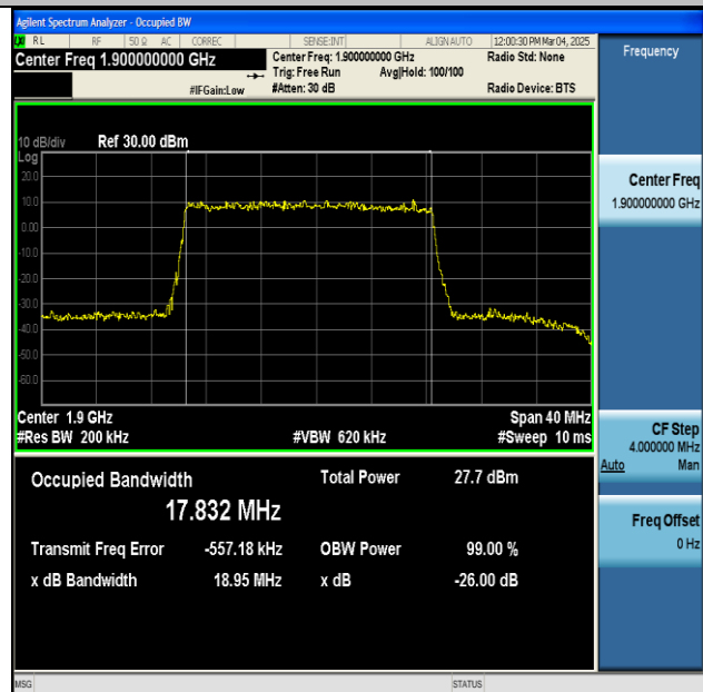
NTNV-n2-PC3-15-20-H-DFT-256QAM-Outer_Full-Ant1-PASS
