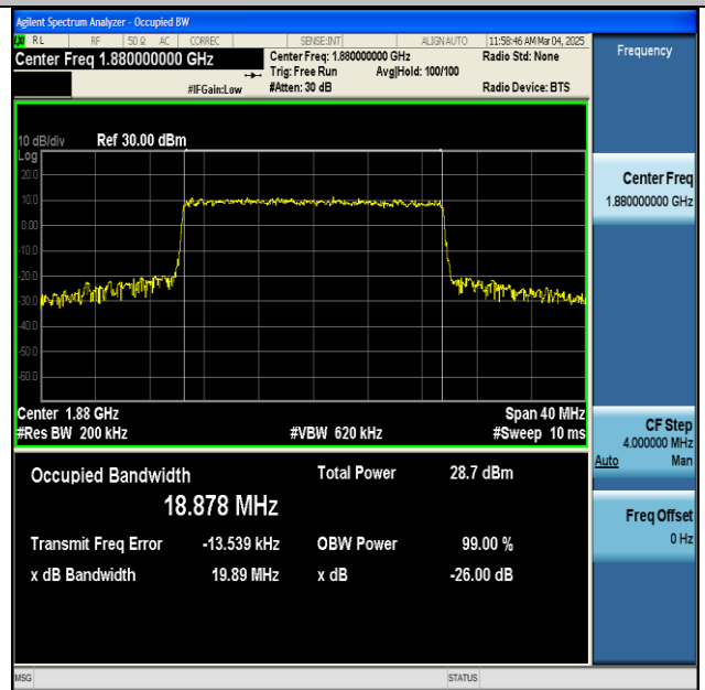
NTNV-n2-PC3-15-20-M-CP-QPSK-Outer_Full-Ant1-PASS
