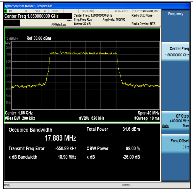
NTNV-n2-PC3-15-20-L-DFT-BPSK-Outer_Full-Ant1-PASS
