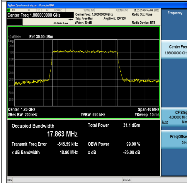
NTNV-n2-PC3-15-20-L-DFT-QPSK-Outer_Full-Ant1-PASS
