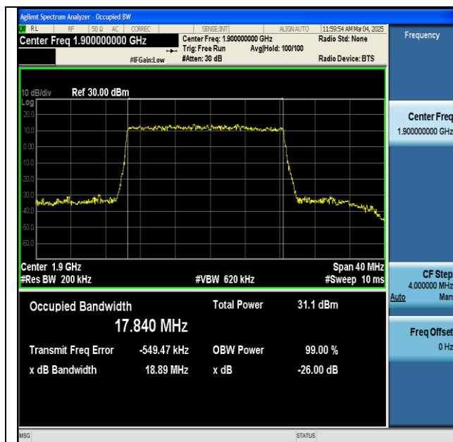
NTNV-n2-PC3-15-20-H-DFT-QPSK-Outer_Full-Ant1-PASS
