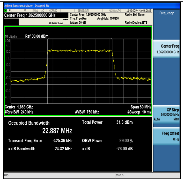
NTNV-n2-PC3-15-25-L-DFT-QPSK-Outer_Full-Ant1-PASS
