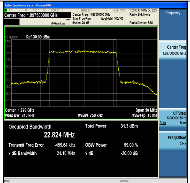
NTNV-n2-PC3-15-25-H-DFT-QPSK-Outer_Full-Ant1-PASS
