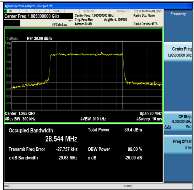
NTNV-n2-PC3-15-30-L-DFT-16QAM-Outer_Full-Ant1-PASS
