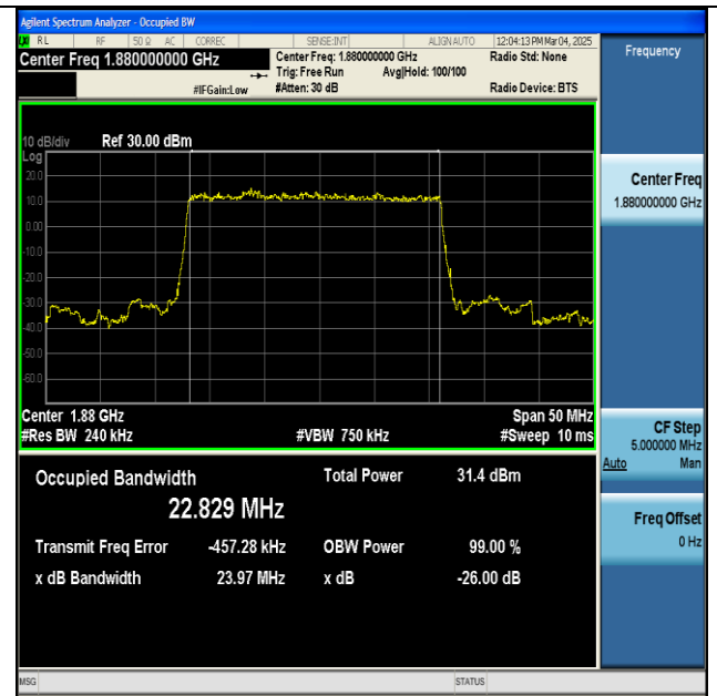
NTNV-n2-PC3-15-25-M-DFT-BPSK-Outer_Full-Ant1-PASS
