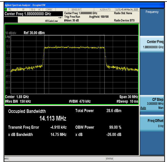
NTNV-n2-PC3-15-15-M-CP-16QAM-Outer_Full-Ant1-PASS
