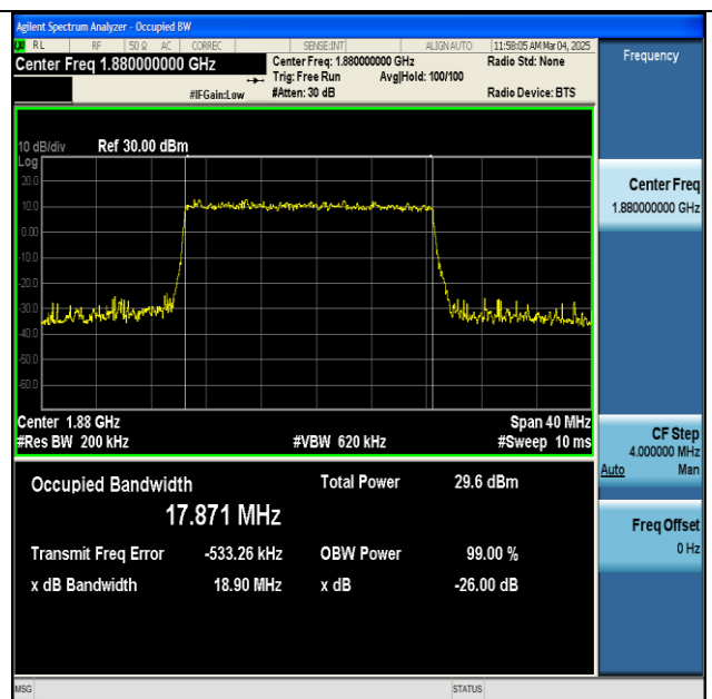
NTNV-n2-PC3-15-20-M-DFT-64QAM-Outer_Full-Ant1- PASS
