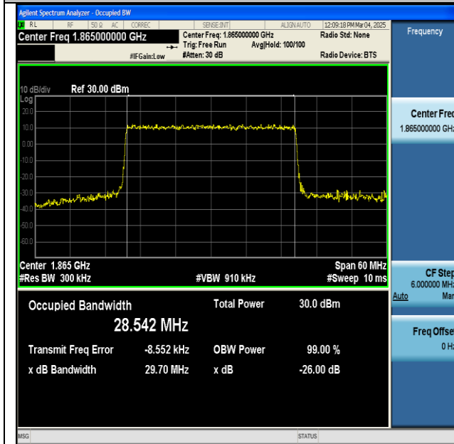
NTNV-n2-PC3-15-30-L-DFT-64QAM-Outer_Full-Ant1-PASS
