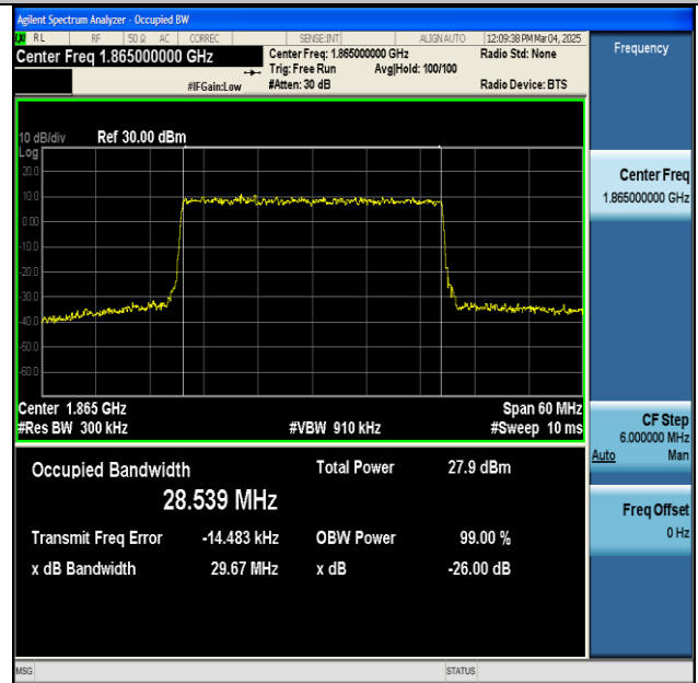
NTNV-n2-PC3-15-30-L-DFT-256QAM-Outer_Full-Ant1-PASS
