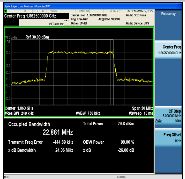
NTNV-n2-PC3-15-25-L-DFT-64QAM-Outer_Full-Ant1- PASS
