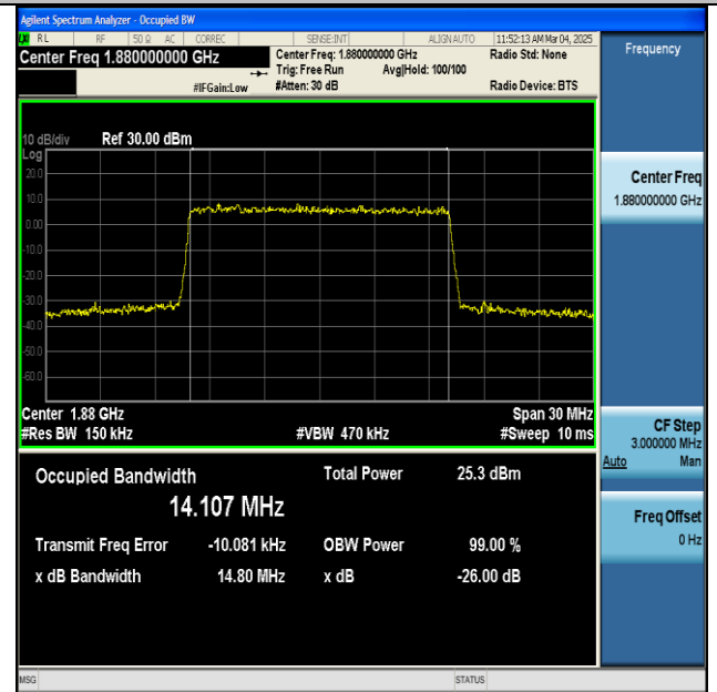
NTNV-n2-PC3-15-15-M-CP-256QAM-Outer_Full-Ant1-PASS
