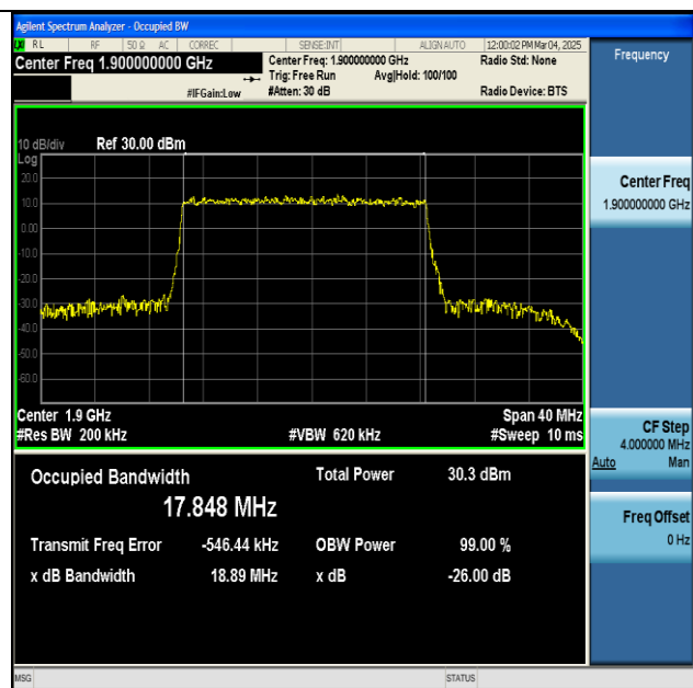
NTNV-n2-PC3-15-20-H-DFT-16QAM-Outer_Full-Ant1-PASS
