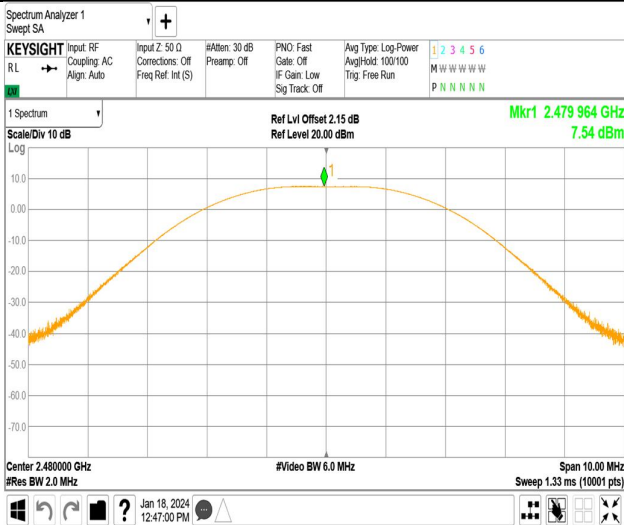
Channel 39 (2480MHz)
