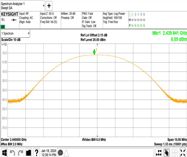
Channel 19 (2440MHz)
