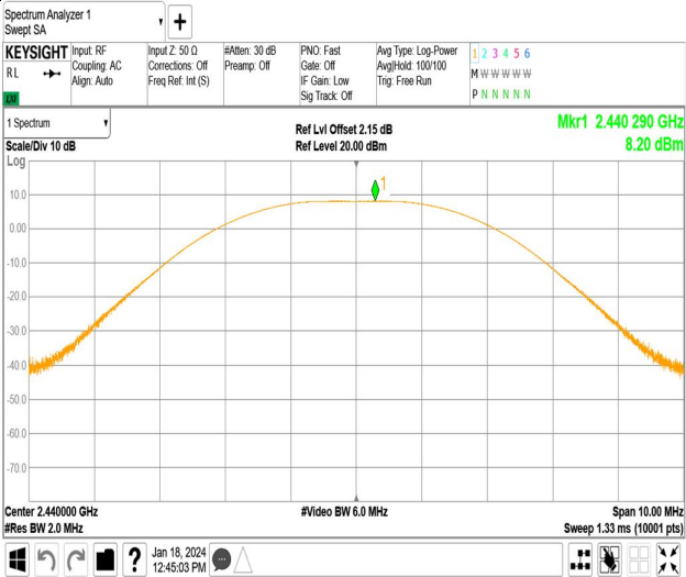
Channel 19 (2440MHz)
