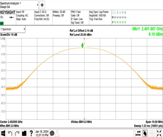
Channel 0 (2402MHz)
