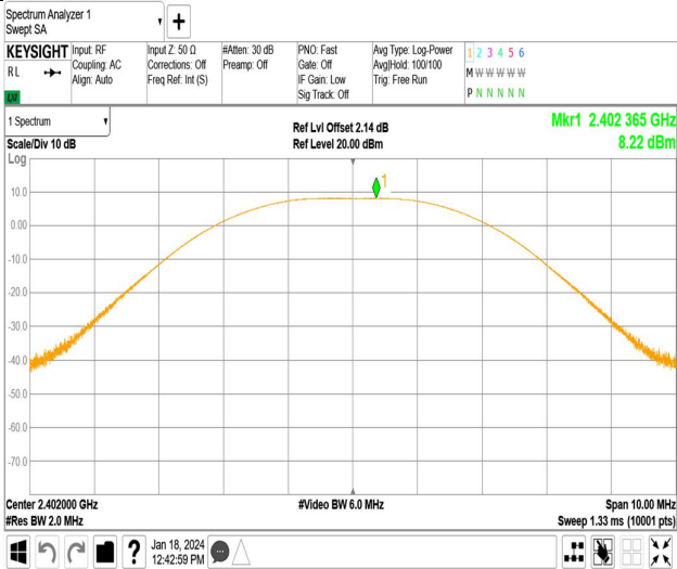
Channel 0 (2402MHz)
