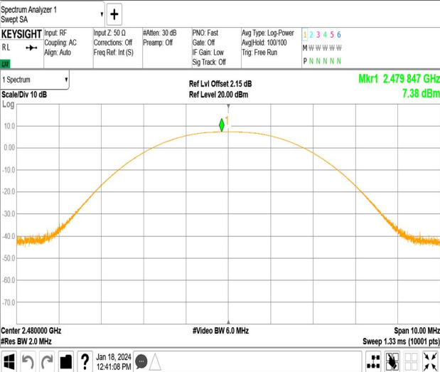
Channel 39 (2480MHz)
