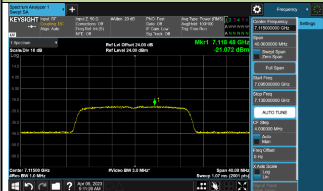
Channel 233 (7115MHz)
