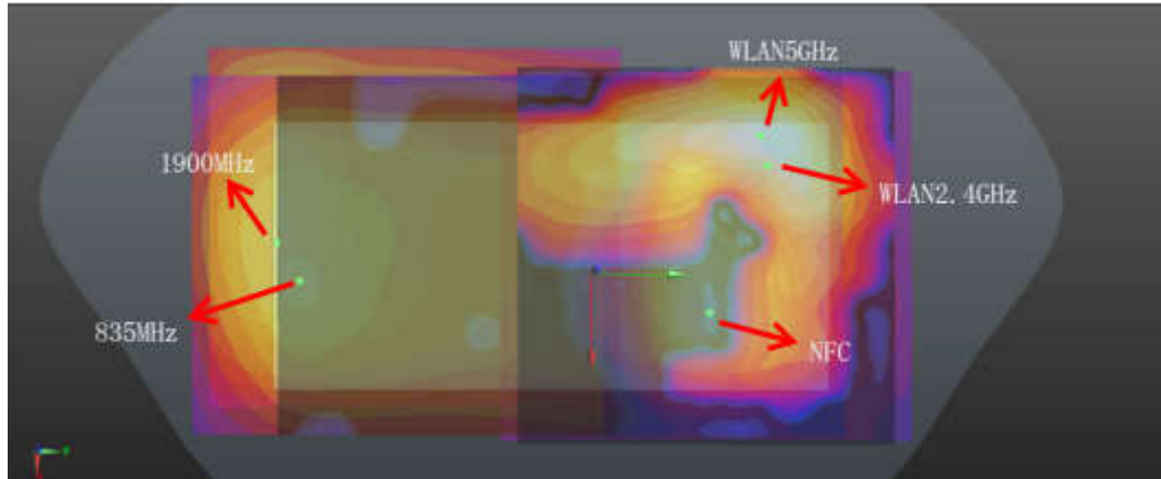
WWAN + WLAN 5GHz/2.4GHz+NFC Back_0mm
