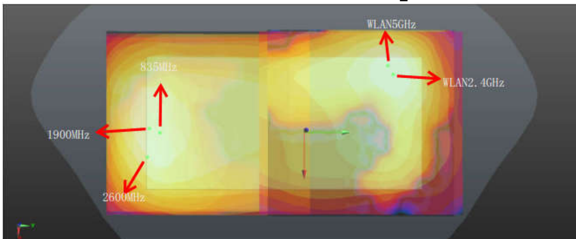
WWAN + WLAN 5GHz/2.4GHz Back_5mm
