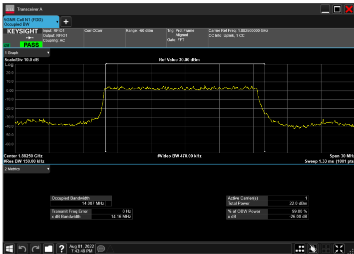
n25_15MHz_15kHz_1882.5MHz_DFT-s-OFDM PI/2 BPSK_RB75@0
