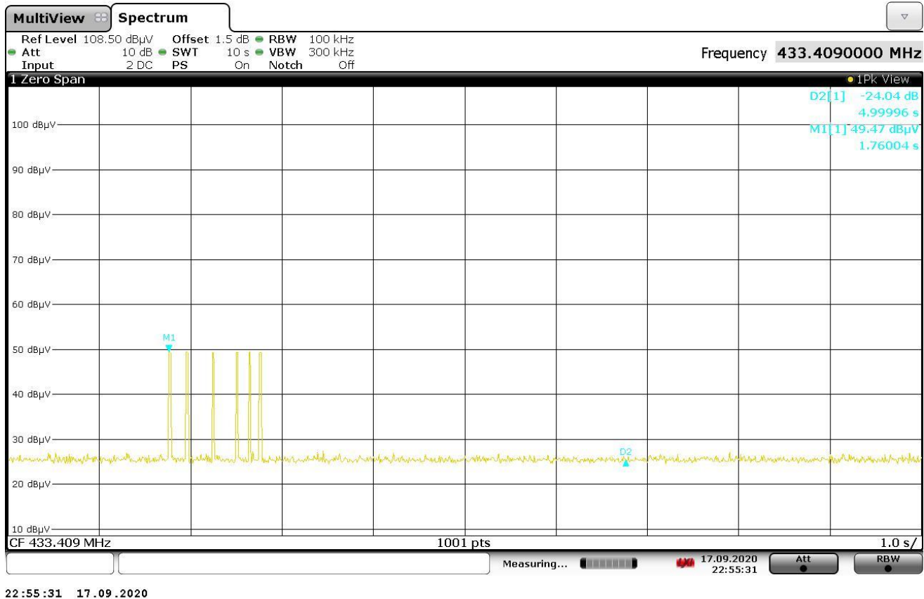
Figure 6 – Supervisory Message TX deactivation
