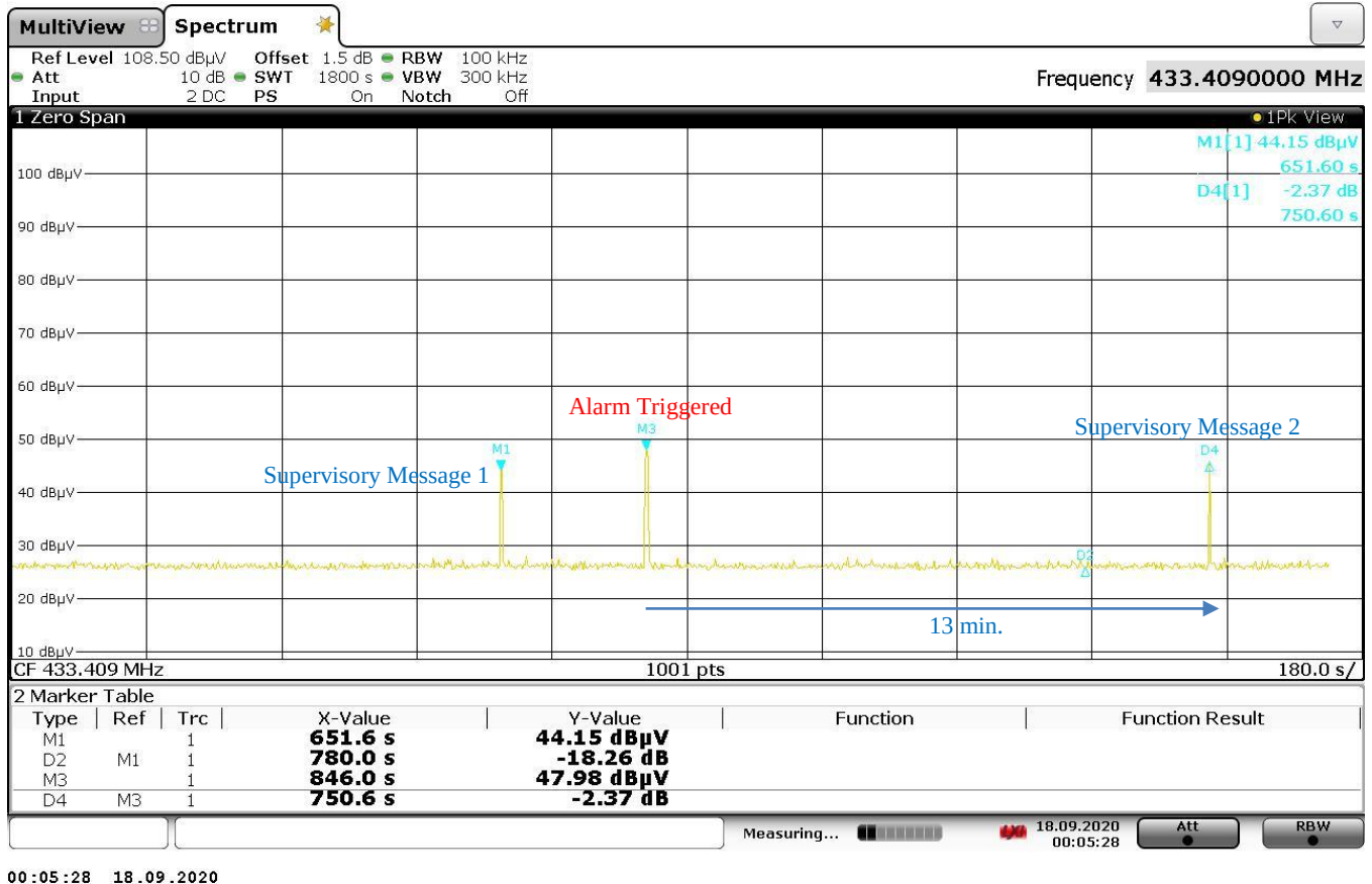
Figure 8 – Alarm event during normal operation
