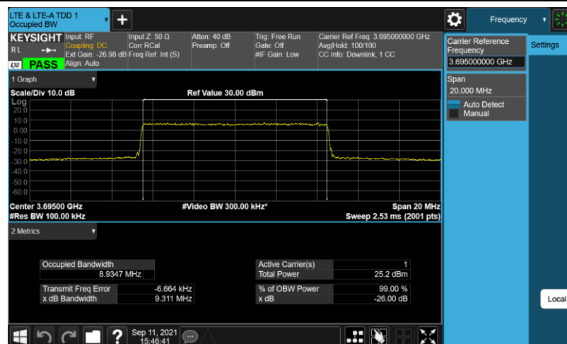
Band48-10MHz-256QAM-56690-E-TM3.1A
