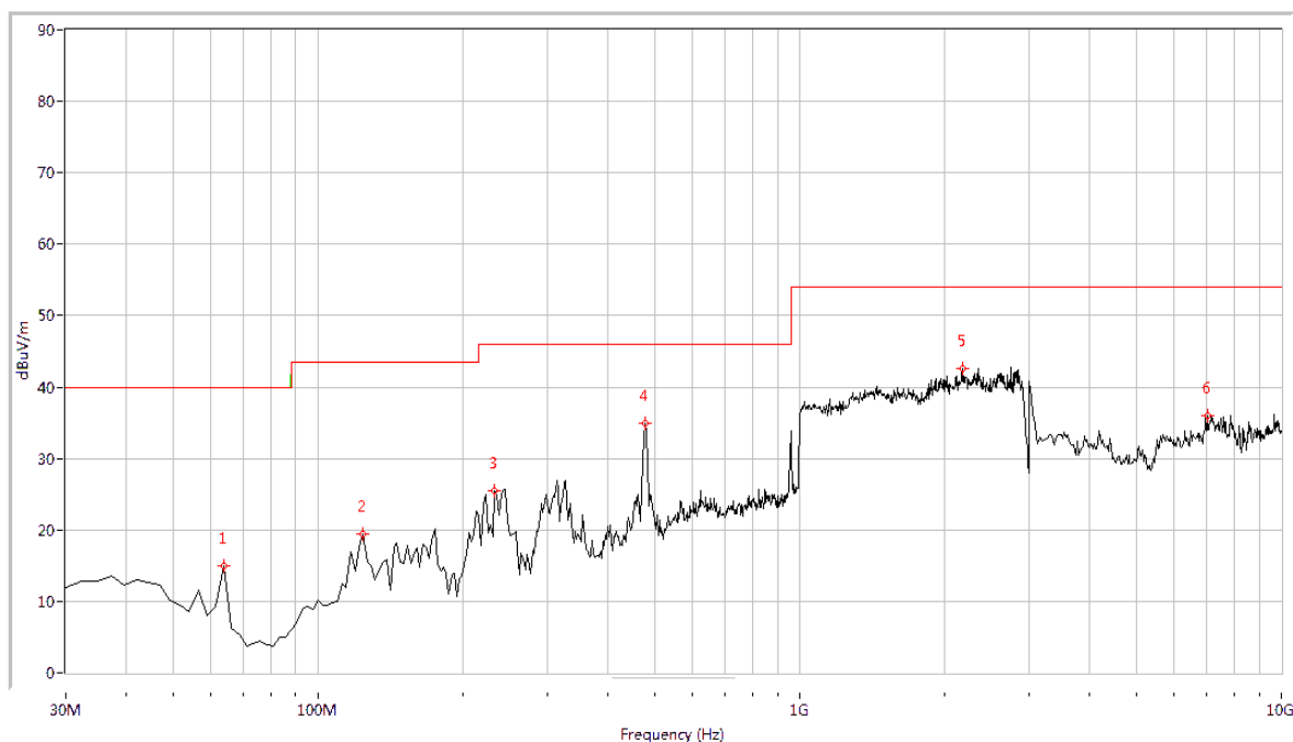
(Plot B: 30MHz – 10GHz, ANT-H)
