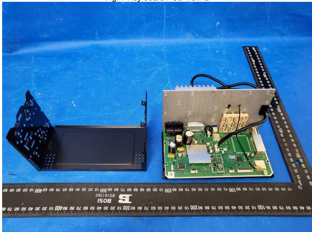
Fig. 8 Internal view-6
