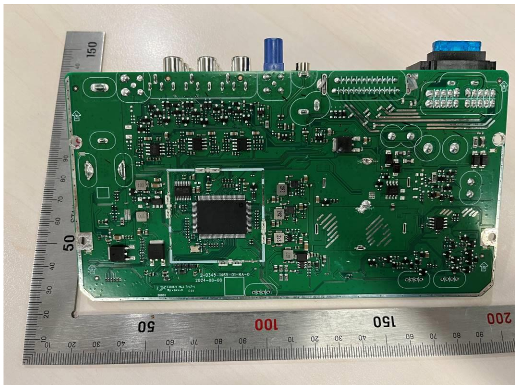
Fig. 14 Main board view-4
