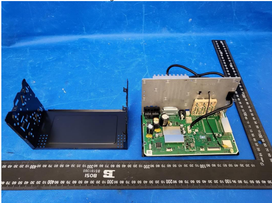
Fig. 2 Internal view-2
