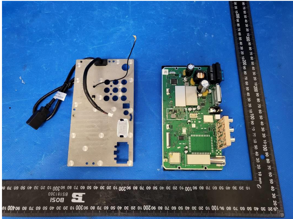
Fig. 9 Internal view-7
