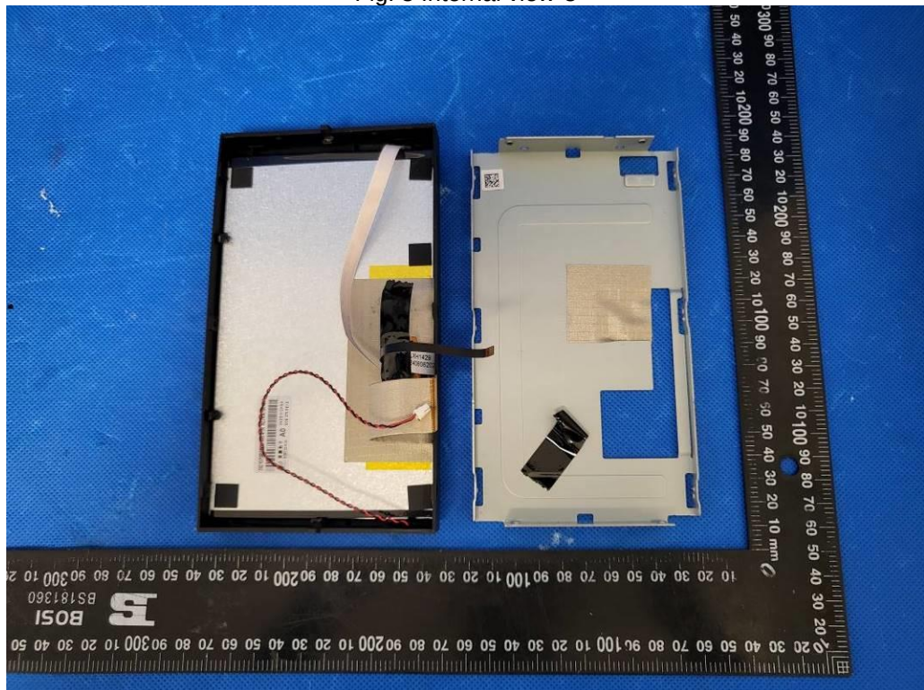
Fig. 4 Internal view-4
