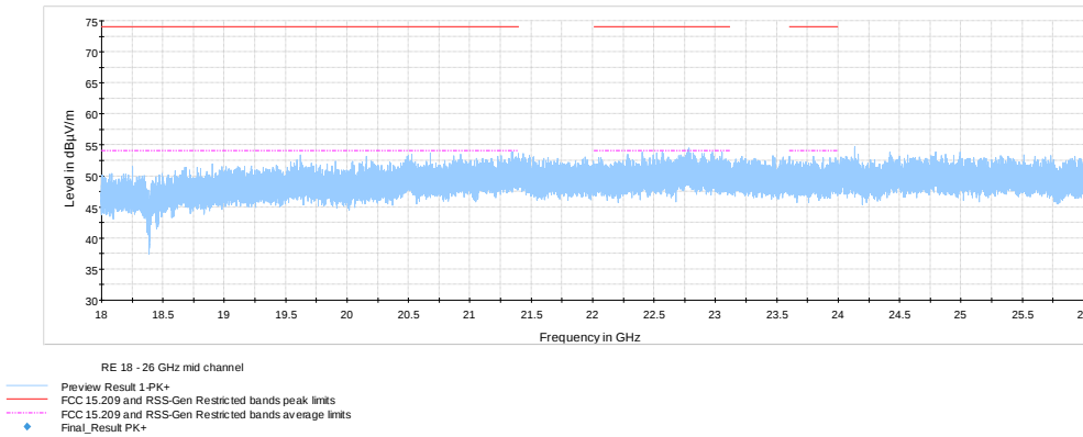
Figure 7.7-13: Radiated spurious emissions on mid channel 18 - 26 GHz
