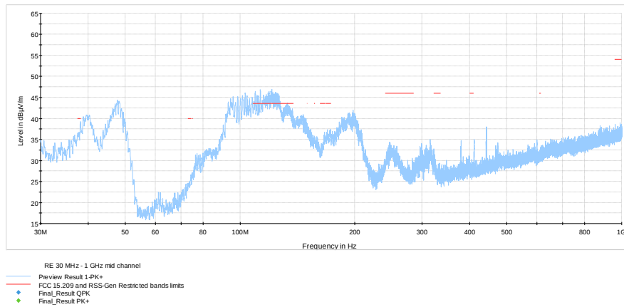
Figure 7.7-7: Radiated spurious emissions on mid channel below 1 GHz
