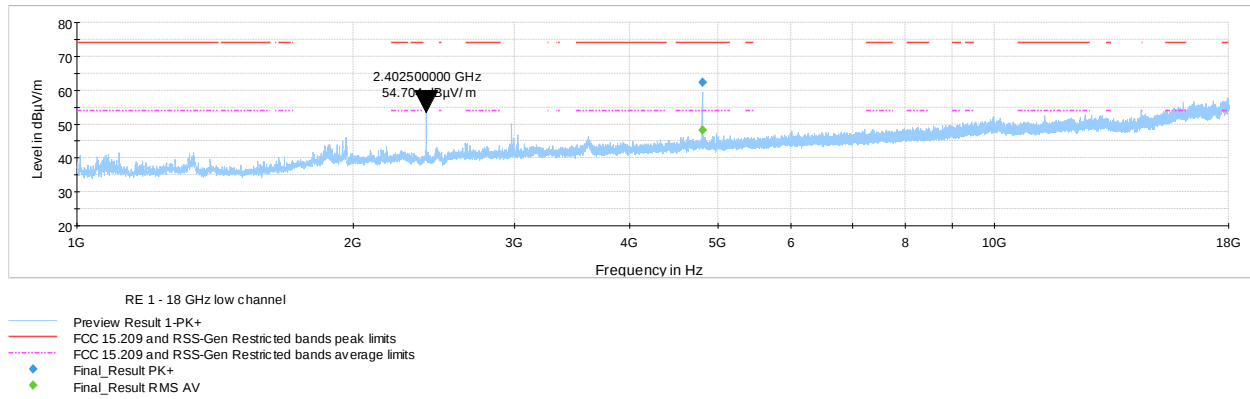
Figure 7.7-9: Radiated spurious emissions on low channel 1 - 18 GHz
