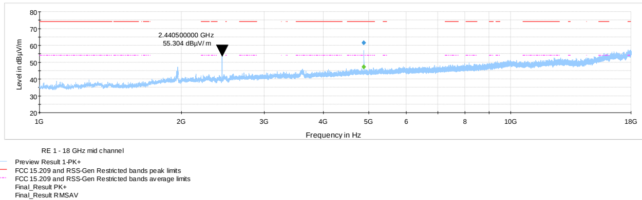
Figure 7.7-10: Radiated spurious emissions on mid channel 1 - 18 GHz
