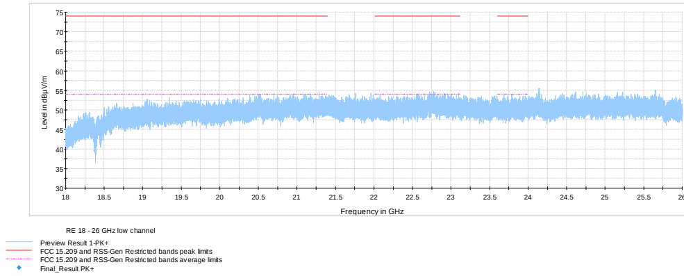
Figure 7.7-12: Radiated spurious emissions on low channel 18 - 26 GHz
