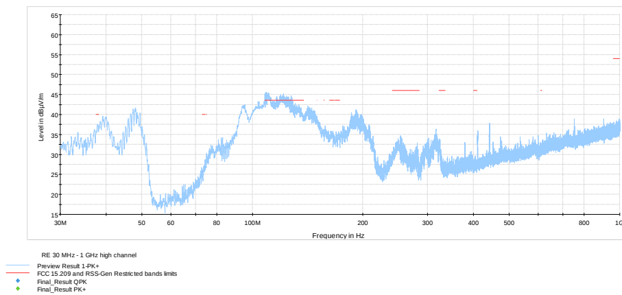
Figure 7.7-8: Radiated spurious emissions on high channel below 1 GHz
