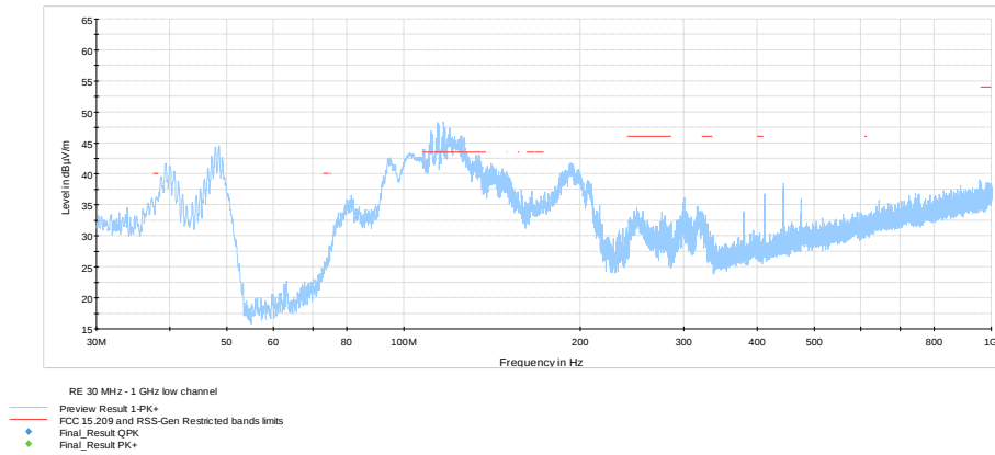
Figure 7.7-6: Radiated spurious emissions on low channel below 1 GHz
