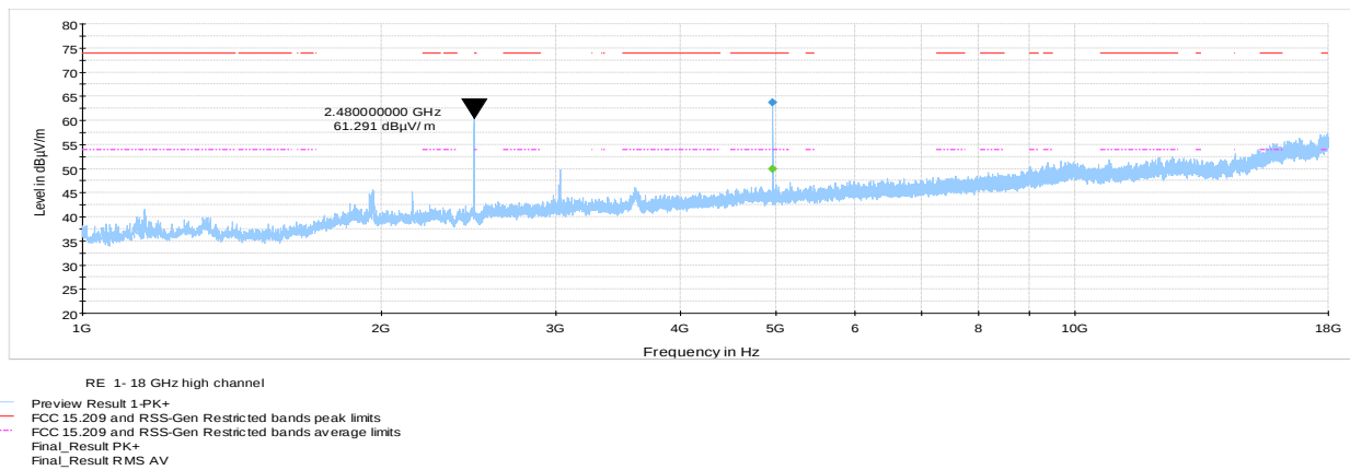
Figure 7.7-11: Radiated spurious emissions on high channel 1 - 18 GHz
