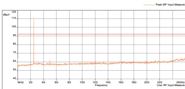
Figure 7.7-5: Conducted spurious emissions on high channel
