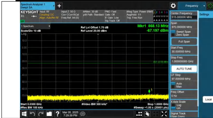
Band4-3MHz-QPSK-19965-1RB#0-30~1000-PASS
