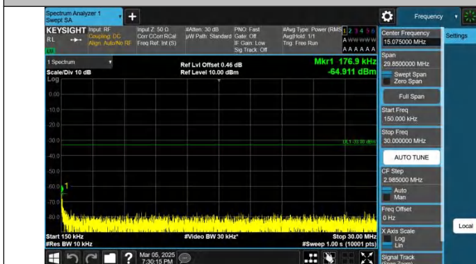
Band4-3MHz-QPSK-19965-1RB#14-0.15~30-PASS
