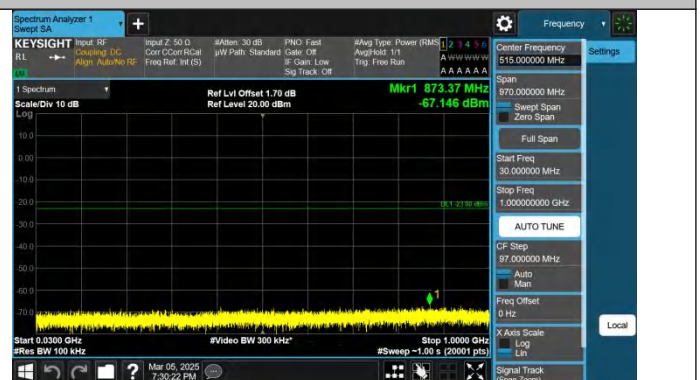
Band4-3MHz-QPSK-19965-1RB#14-30~1000-PASS
