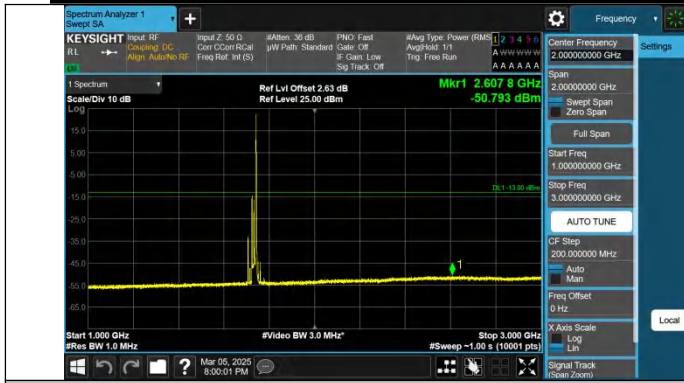
Band4-20MHz-QPSK-20175-1RB#99-1000~3000-PASS
