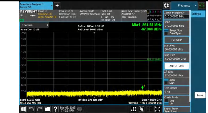
Band4-10MHz-QPSK-20000-1RB#49-30~1000-PASS
