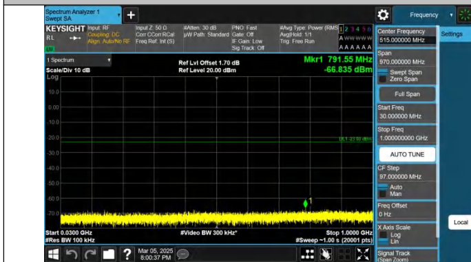
Band4-20MHz-QPSK-20300-1RB#0-30~1000-PASS
