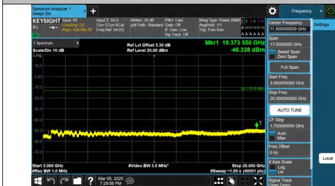
Band4-3MHz-QPSK-19965-1RB#0-3000~20000-PASS
