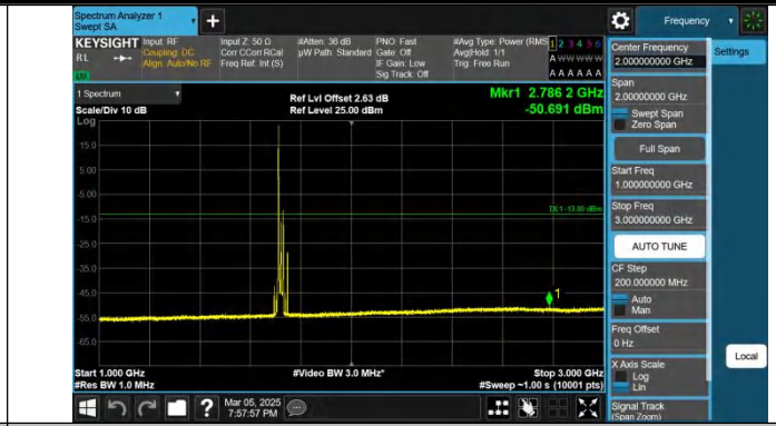
Band4-20MHz-QPSK-20050-1RB#0-1000~3000-PASS
