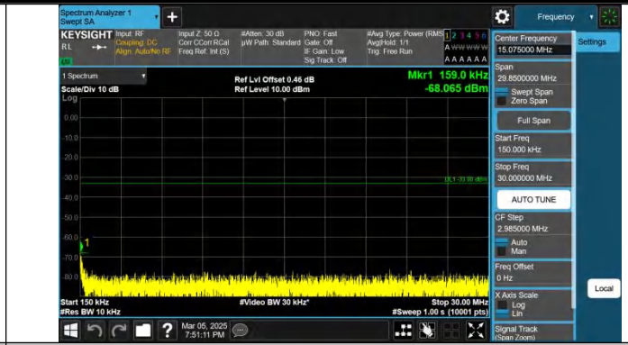
Band4-15MHz-QPSK-20025-1RB#0-0.15~30-PASS
