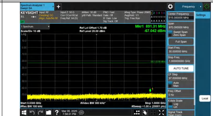
Band4-20MHz-QPSK-20050-1RB#99-30~1000-PASS
