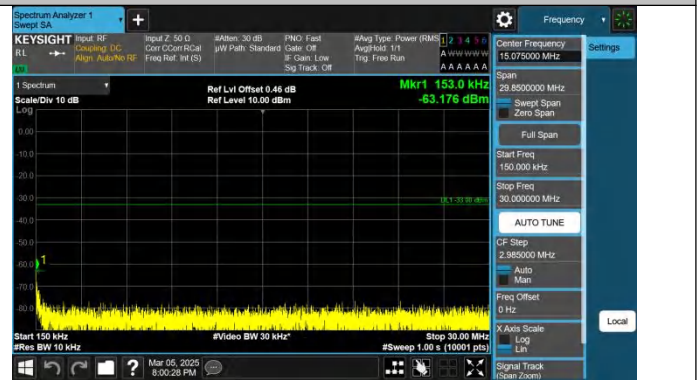
Band4-20MHz-QPSK-20300-1RB#0-0.15~30-PASS
