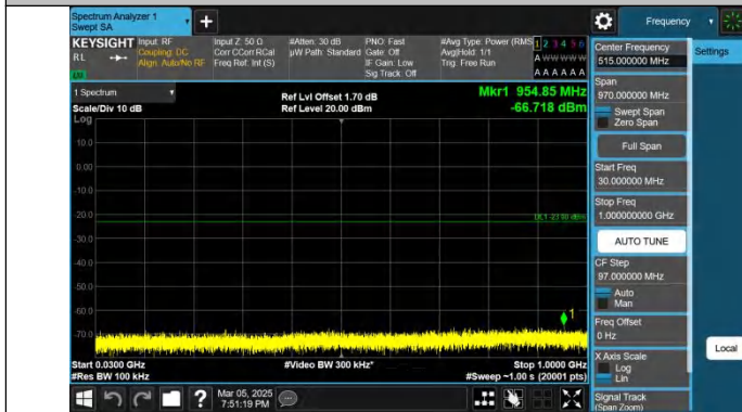
Band4-15MHz-QPSK-20025-1RB#0-30~1000-PASS
