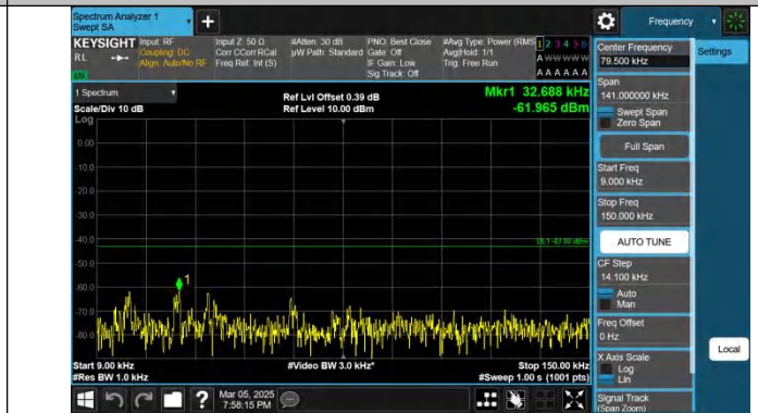
Band4-20MHz-QPSK-20050-1RB#99-0.009~0.15-PASS
