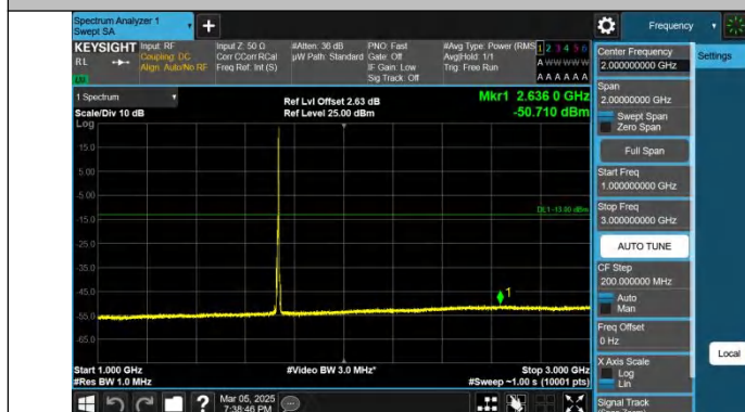
Band4-5MHz-QPSK-20175-1RB#24-1000~3000-PASS
