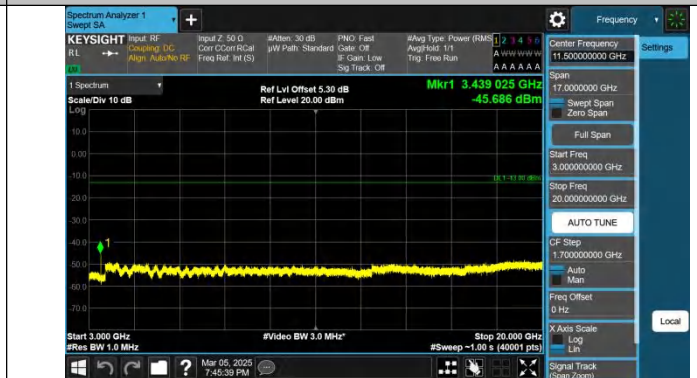
Band4-10MHz-QPSK-20000-1RB#49-3000~20000-PASS
