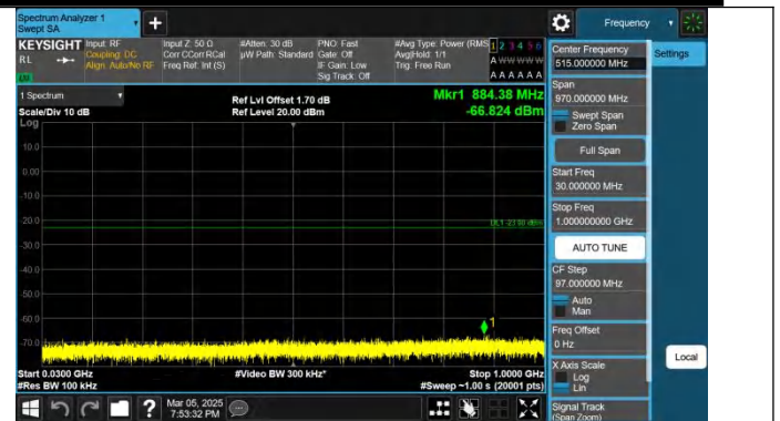
Band4-15MHz-QPSK-20175-1RB#74-30~1000-PASS
