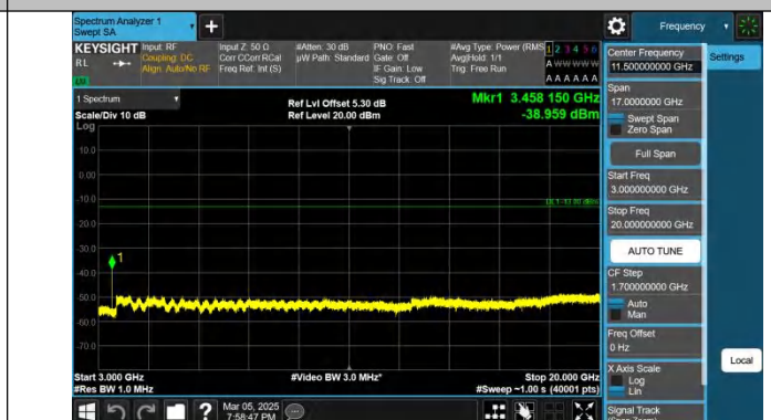
Band4-20MHz-QPSK-20050-1RB#99-3000~20000-PASS
