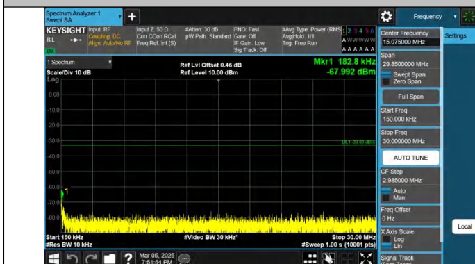
Band4-15MHz-QPSK-20025-1RB#74-0.15~30-PASS
