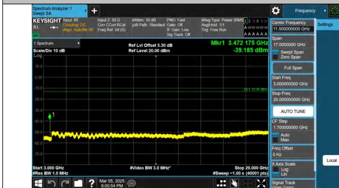
Band4-20MHz-QPSK-20300-1RB#0-3000~20000-PASS
