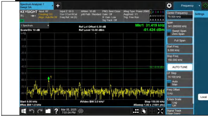
Band4-15MHz-QPSK-20025-1RB#0-0.009~0.15-PASS
