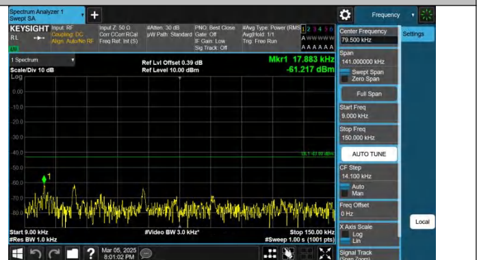
Band4-20MHz-QPSK-20300-1RB#99-0.009~0.15-PASS
