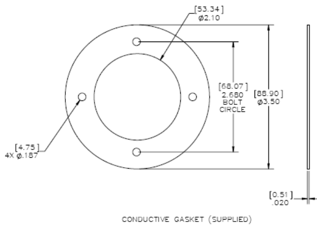
Figure 4-3 - Iridium Antenna, Gasket
