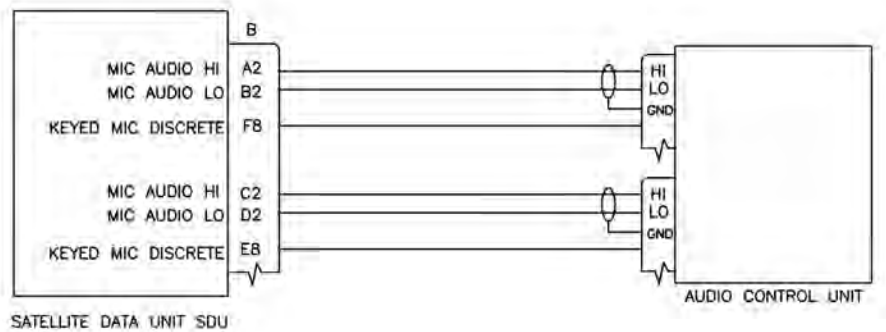
Figure 6-7 – Latched ACP Audio Interface
