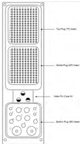
Figure 3-9 – SDU Connector Map
