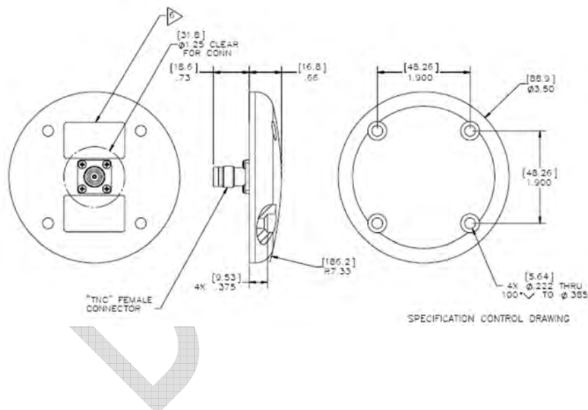
Figure 4-2 - Iridium Antenna, Outline and Dimensions
