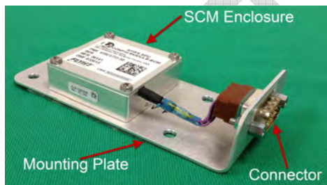
Figure 3-3 –Iridium SATCOM System SDU Configuration Module (SCM)
