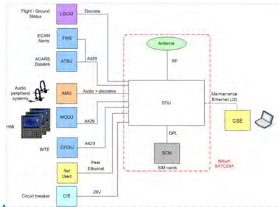
Figure 2-3 –Iridium SATCOM System External Interfaces NEED EFB GRAPHIC
