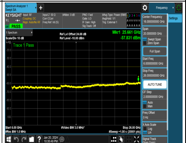
NTNV_N48_PC3_30_40_H_TID4_NS_01_6000_26000_#1
