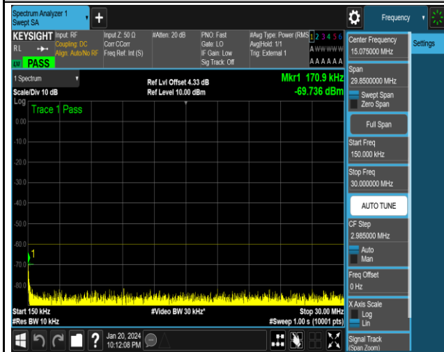
NTNV_N48_PC3_30_40_H_TID1_NS_01_0.15_30_#1
