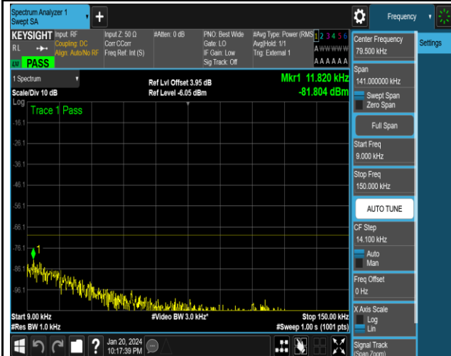
NTNV_N48_PC3_30_40_H_TID2_NS_01_0.009_0.15_#1
