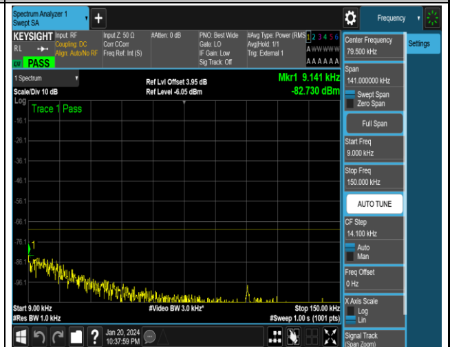
NTNV_N48_PC3_30_40_H_TID5_NS_01_0.009_0.15_#1
