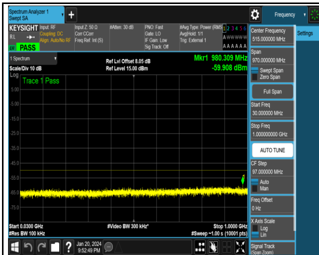
NTNV_N48_PC3_30_40_M_TID16_NS_01_30_1000_#1
