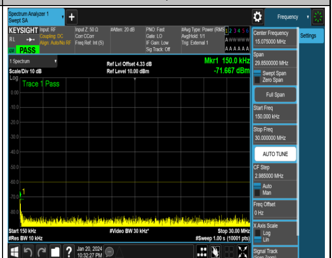
NTNV_N48_PC3_30_40_H_TID4_NS_01_0.15_30_#1
