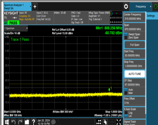
NTNV_N48_PC3_30_40_H_TID2_NS_01_30_1000_#1
