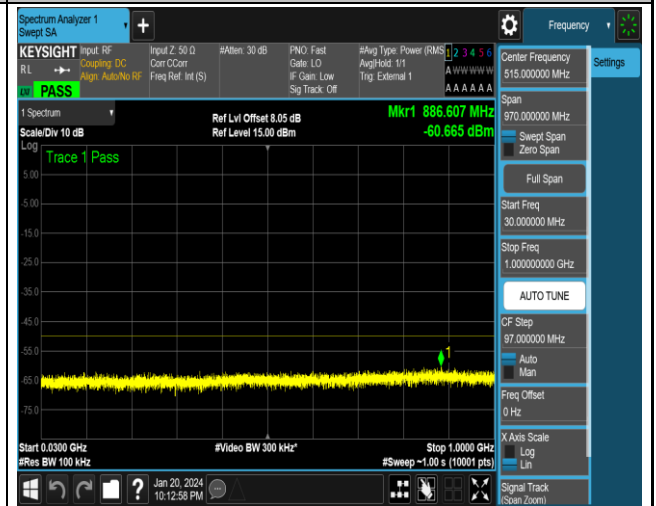
NTNV_N48_PC3_30_40_H_TID1_NS_01_30_1000_#1
