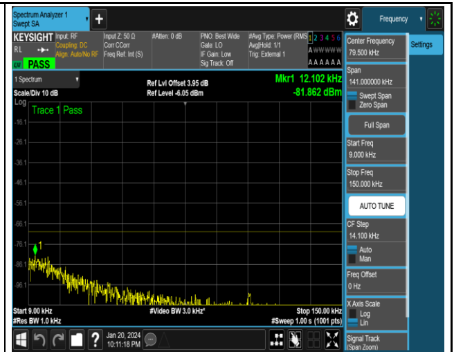
NTNV_N48_PC3_30_40_H_TID1_NS_01_0.009_0.15_#1
