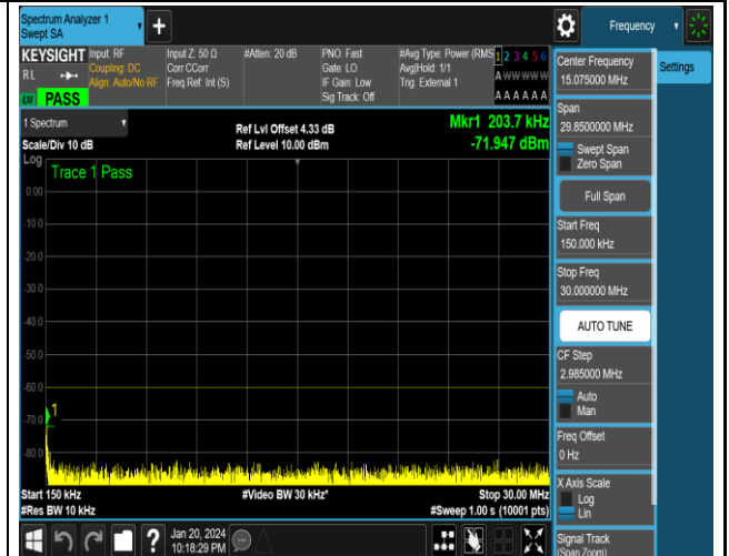
NTNV_N48_PC3_30_40_H_TID2_NS_01_0.15_30_#1
