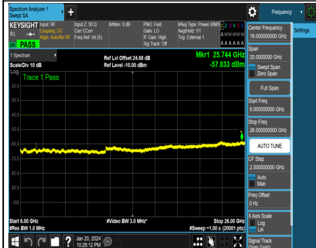
NTNV_N48_PC3_30_40_H_TID3_NS_01_6000_26000_#1
