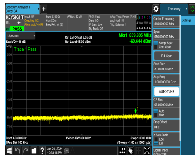
NTNV_N48_PC3_30_40_H_TID4_NS_01_30_1000_#1
