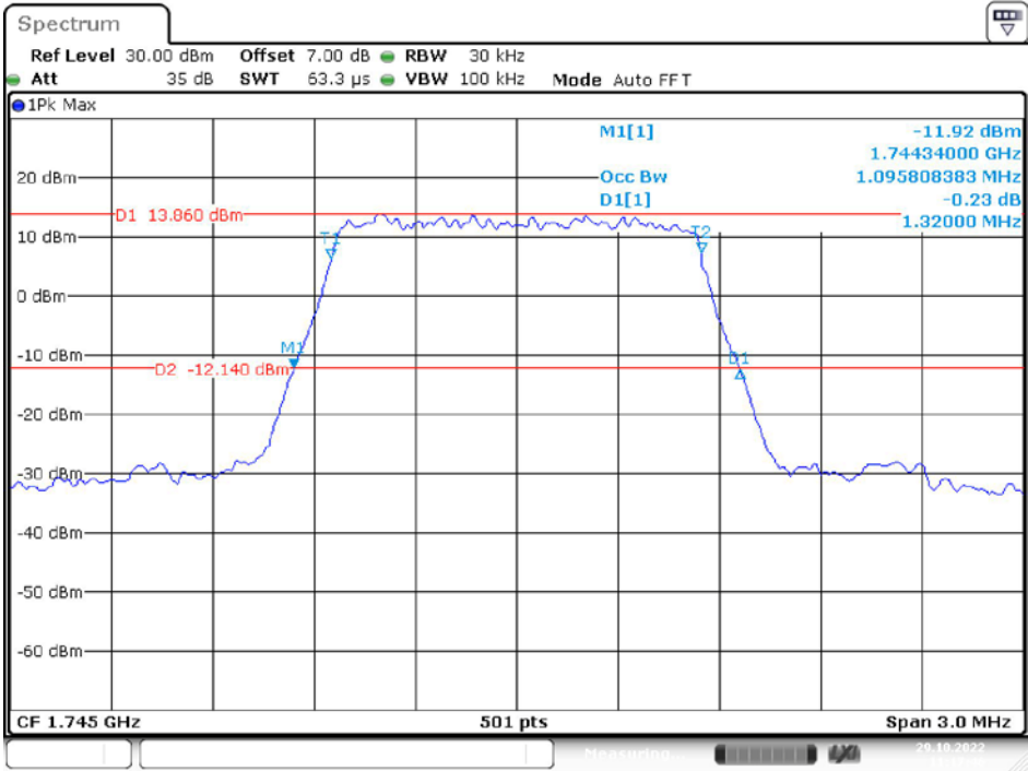
Band 66_1.4 MHz_Middle_16QAM_RB6#0
