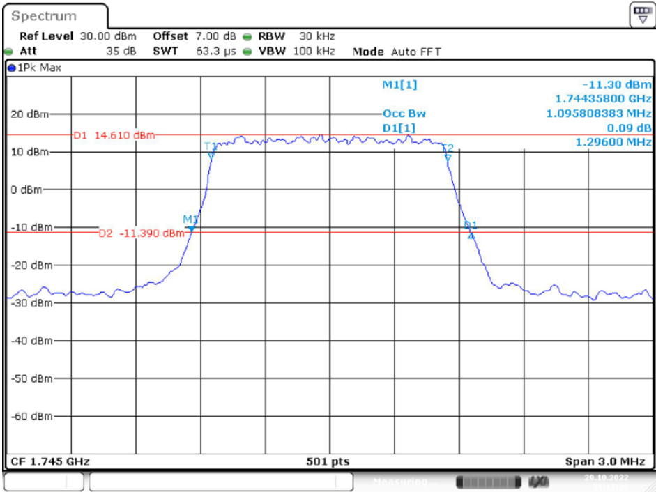
Band 66_1.4 MHz_Middle_QPSK_RB6#0
