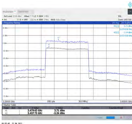
1-N78-3450-3550--30-100-M-1-DFT-256QAM-Outer_Full-270@0-Ant0-9.25-100%-0.00-9.25-PASS-≤13
