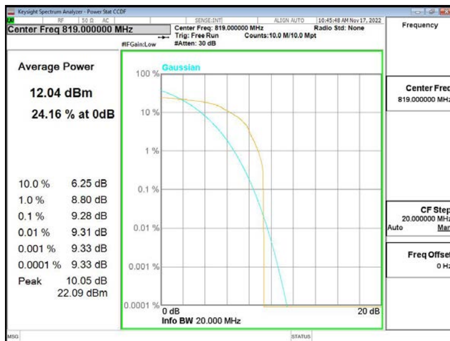
Band26-CH26740-819MHz-10MHz Bandwidth-16QAM
