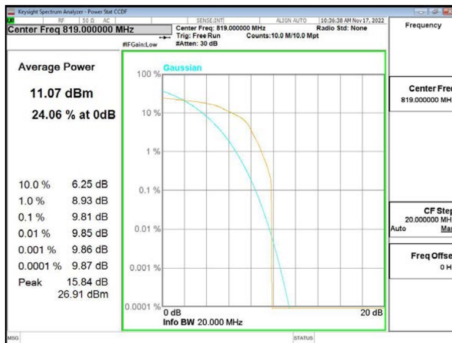
Band26-CH26740-819MHz-1.4MHz Bandwidth-16QAM
