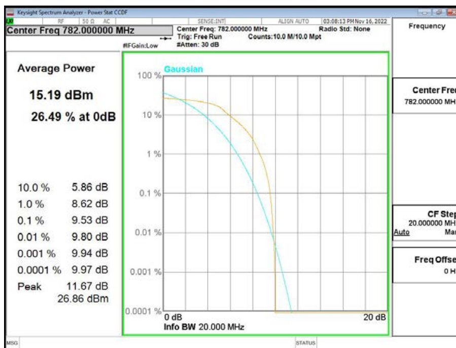
Band13-CH23230-782MHz-5MHz Bandwidth-QPSK
