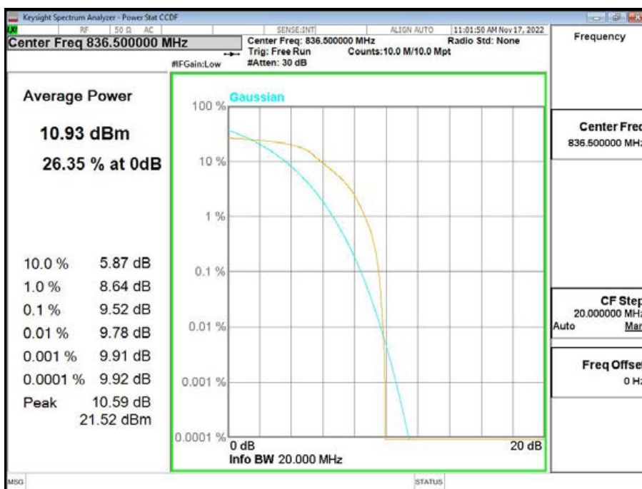
Band26-CH26915-836.5MHz-10MHz Bandwidth-QPSK
