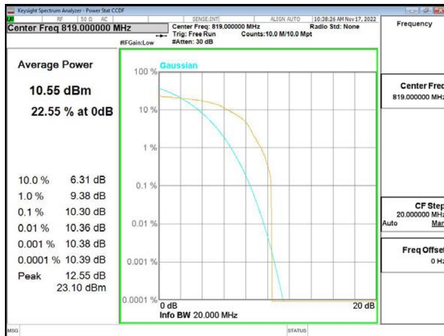
Band26-CH26740-819MHz-3MHz Bandwidth-16QAM
