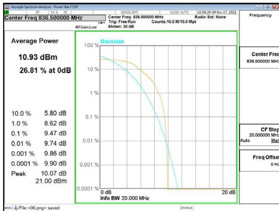
Band26-CH26915-836.5MHz-5MHz Bandwidth-QPSK
