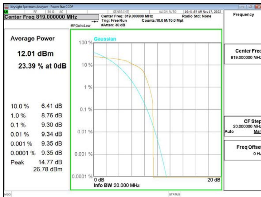
Band26-CH26740-819MHz-5MHz Bandwidth-16QAM
