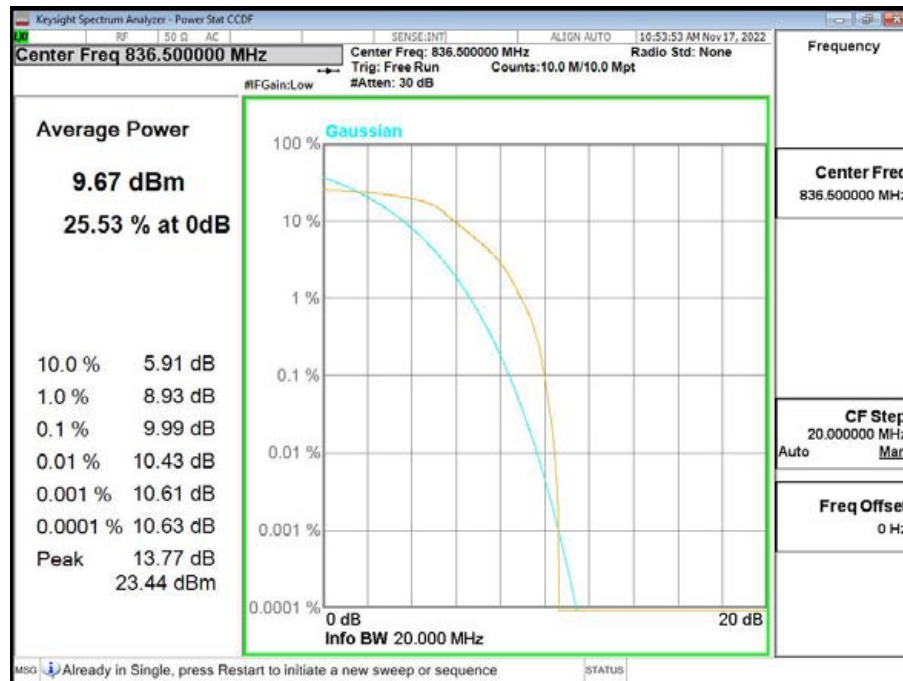
Band26-CH26915-836.5MHz-1.4MHz Bandwidth-QPSK
