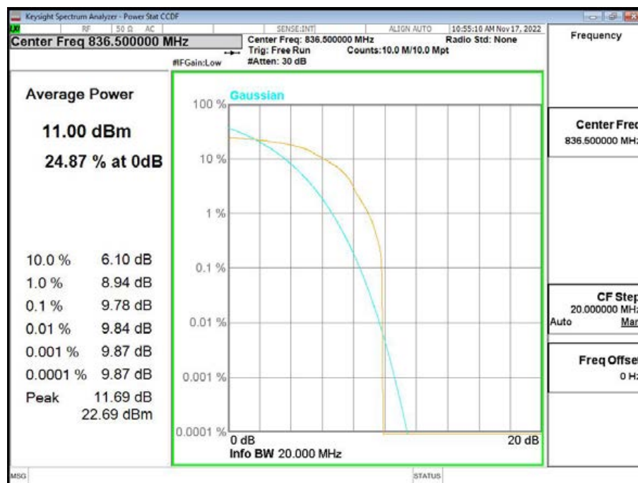
Band26-CH26915-836.5MHz-1.4MHz Bandwidth-16QAM
