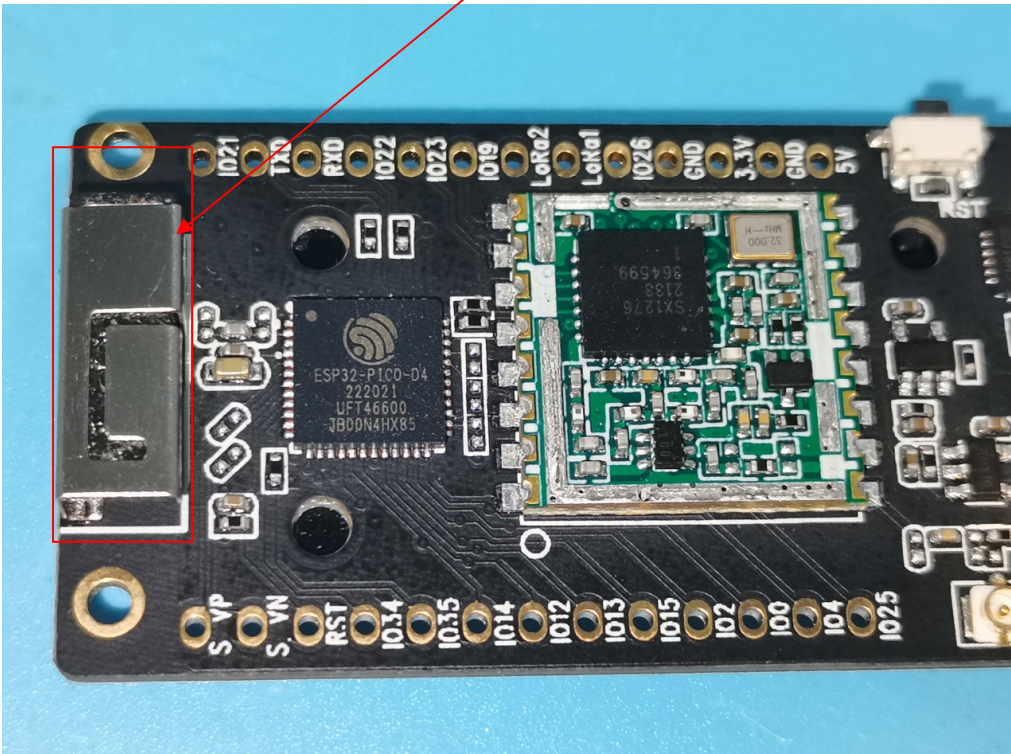
BT/Wi-Fi Antenna
