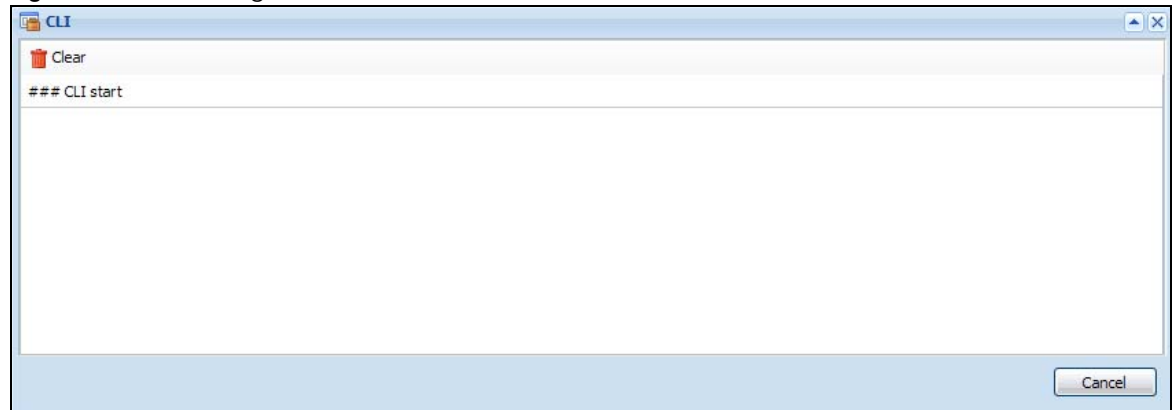
Figure 15 CLI Messages
