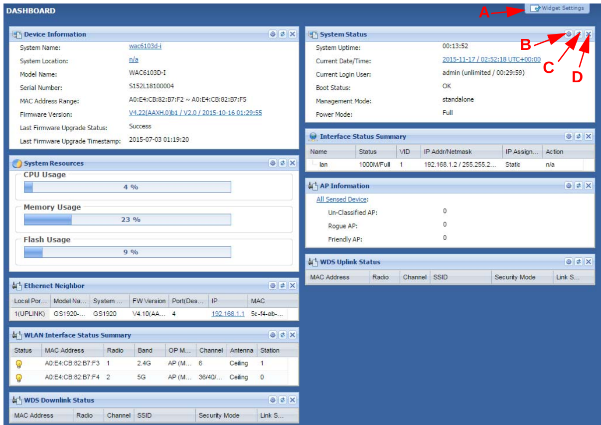
Figure 19 Dashboard
