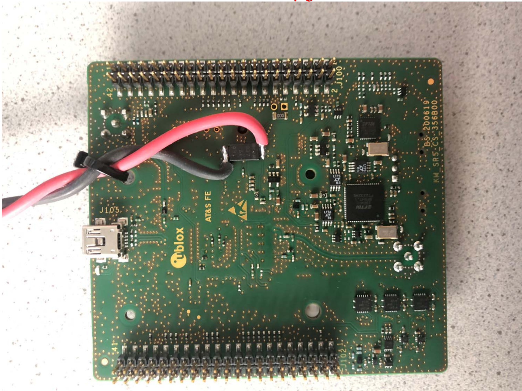
Back side of module test jig.
