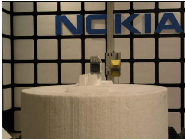
RF Output power measurement
