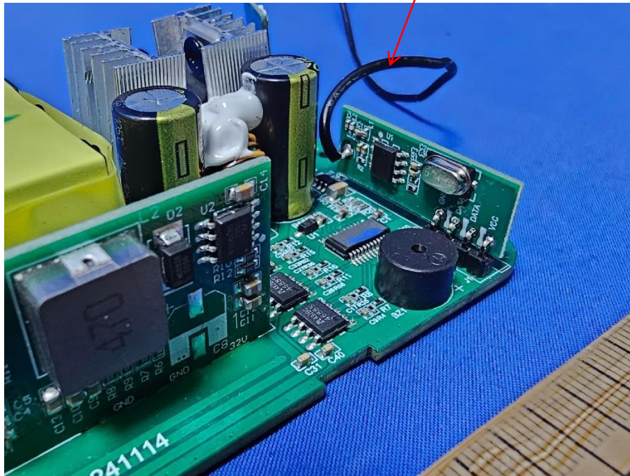
433.92 receiving antenna
