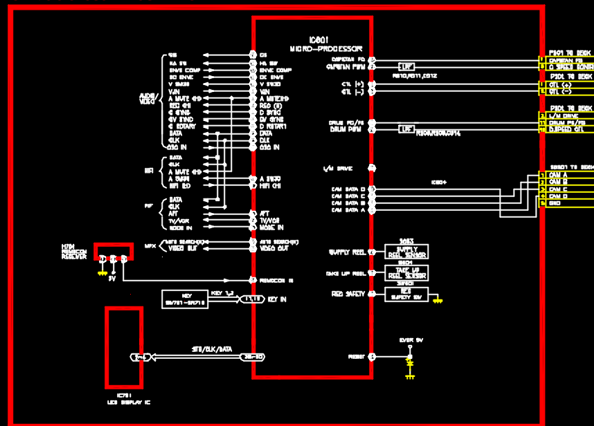
SERVO & SYSCON BLOCK DIAGRAM
