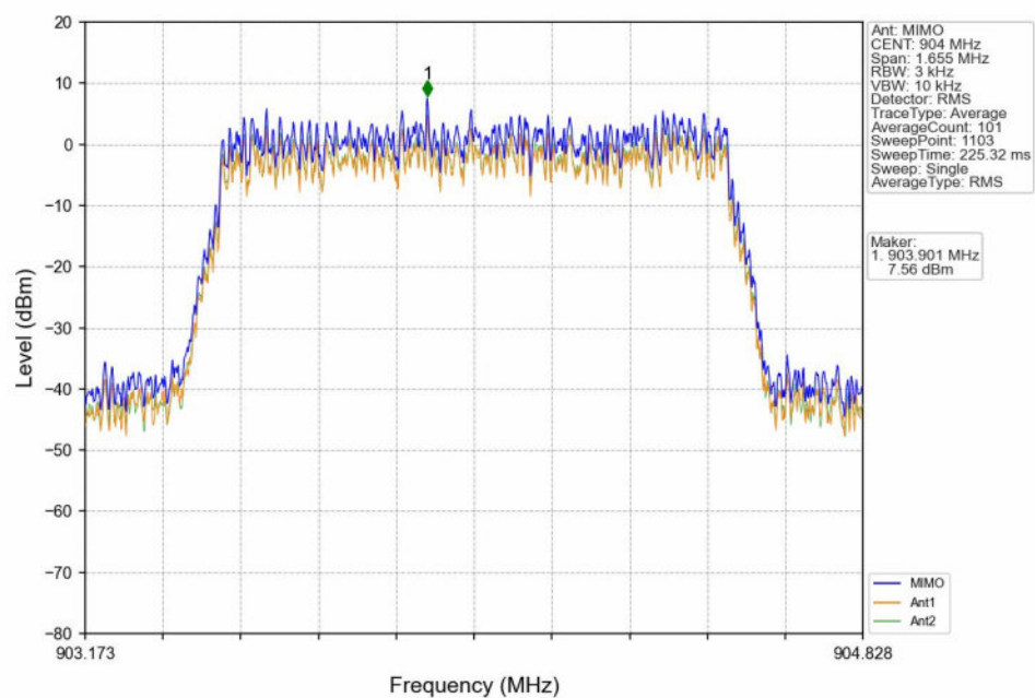
16QAM_LCH_904MHz_MIMO_NTNV
