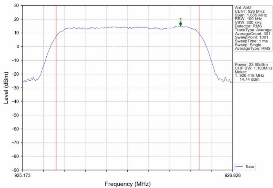
QPSK_HCH_926MHz_Ant2_NTNV
