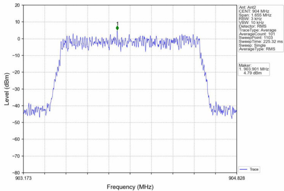
16QAM_LCH_904MHz_MIMO_NTNV
