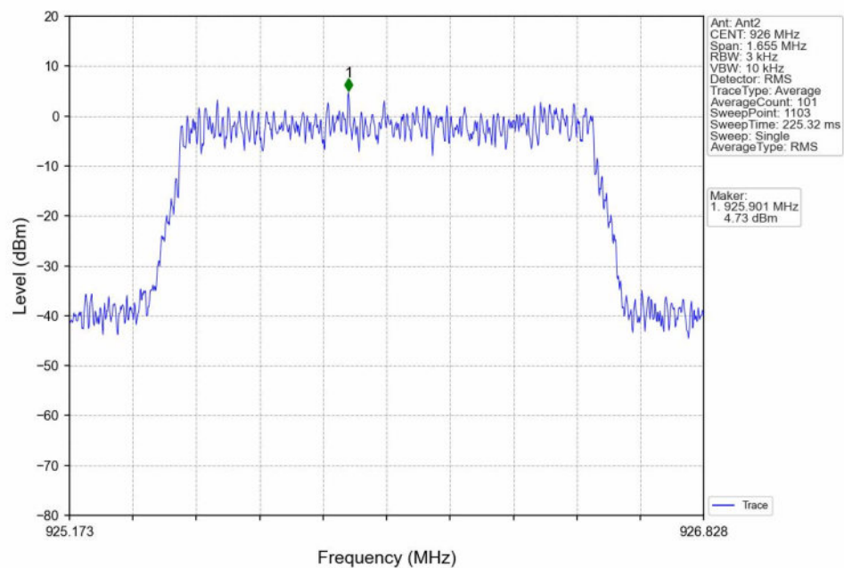
QPSK_HCH_926MHz_Ant2_NTNV
