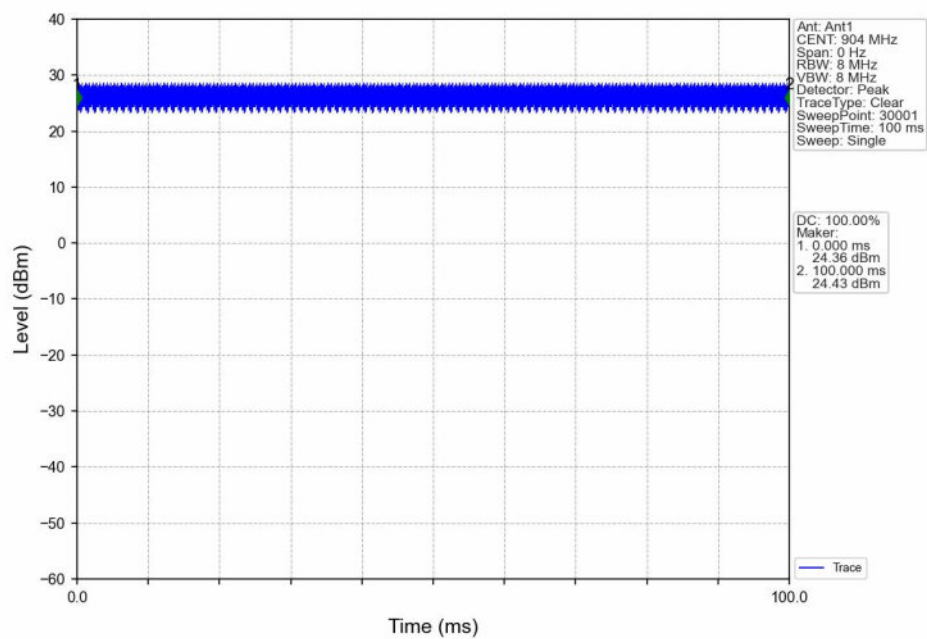
16QAM_LCH_904MHz_Ant1_NTNV
