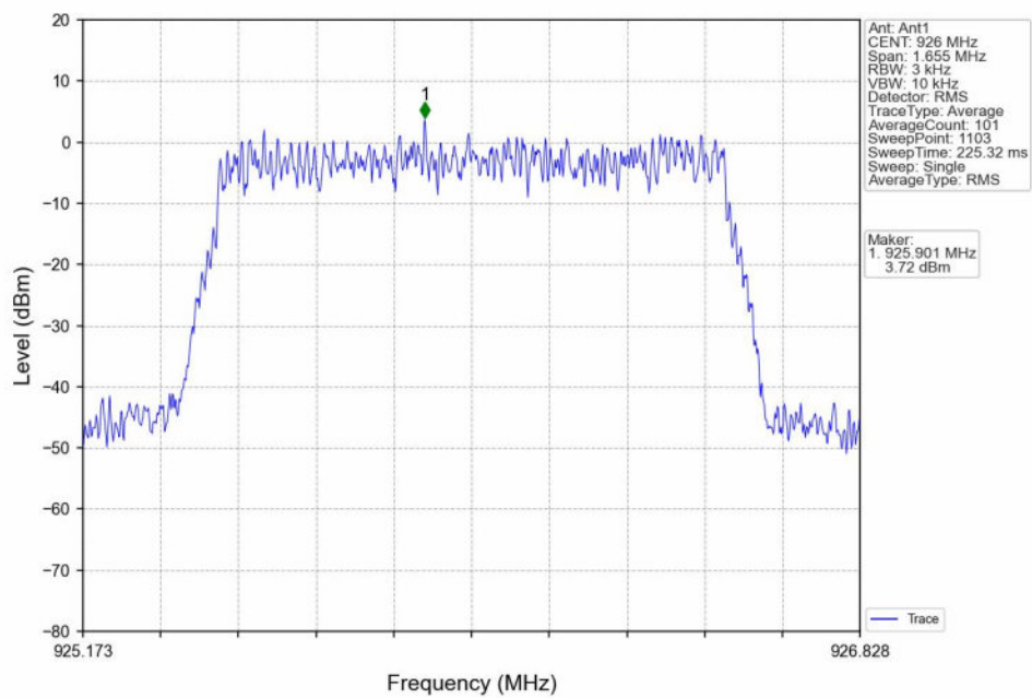
16QAM_HCH_926MHz_Ant1_NTNV
