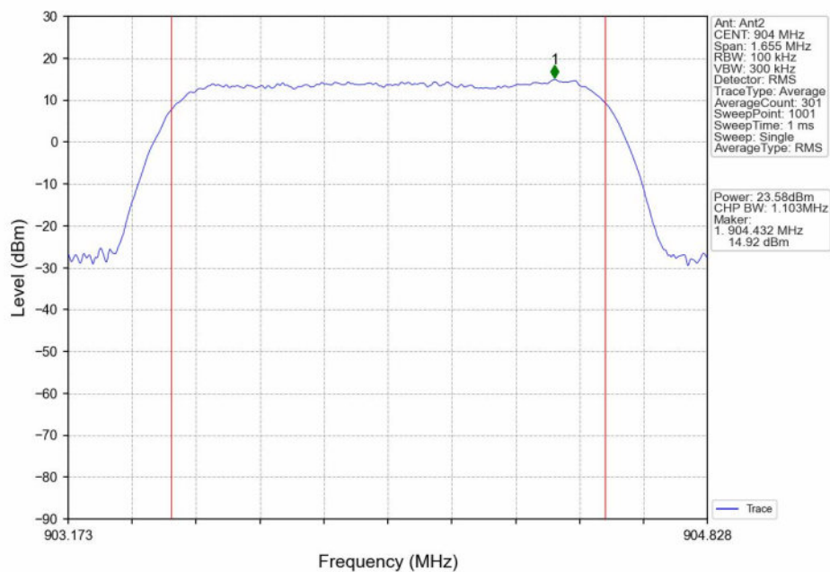
16QAM_LCH_904MHz_Ant2_NTNV
