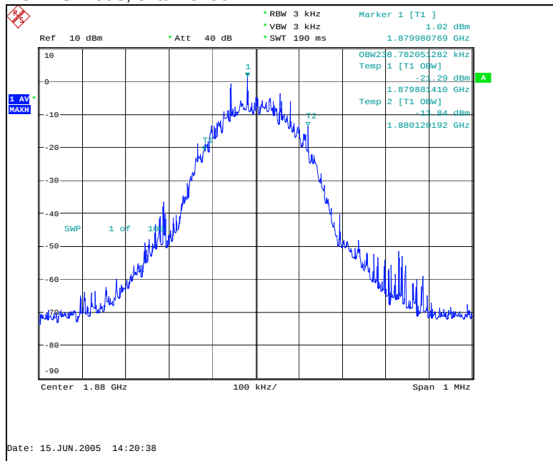
EGPRS mode, channel 661
